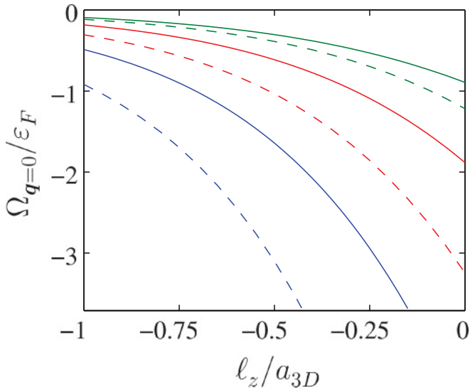
FIG. 2. (Color online) Binding energy of molecules at zero temperature for \epsilon_F/\hbar\omega_z = 0.025, 0.075, and 0.2 (from bottom to top). The binding energy in the presence of Fermi sea (solid lines) is smaller than the vacuum binding energy (dashed line) for the parameters considered.
