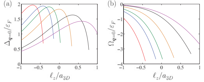
FIG. 1. (Color online) Growth rate of the pairing instability (a) and the binding energy of molecules (b) at zero temperature as a function of \ell_z/a_{3D} . The values of \varepsilon_F/\hbar\omega_z are (from left to right) \varepsilon_F/\hbar\omega_z = 0.0175, 0.025, 0.0375, 0.075, 0.2, and 0.4 .
