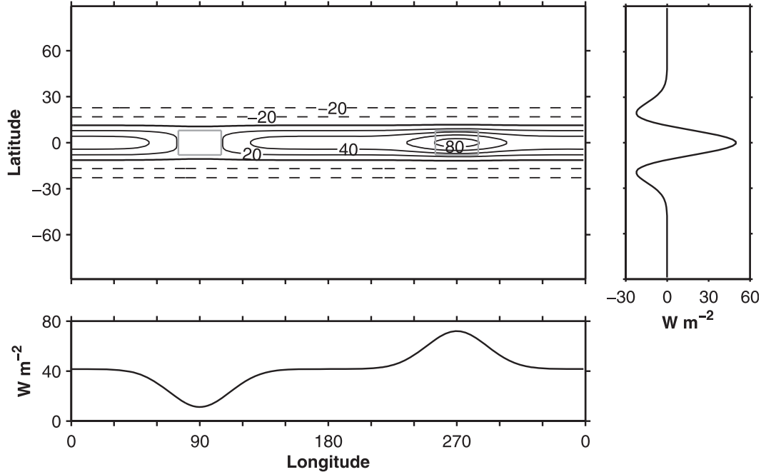
FIG. 1. Ocean energy flux divergence, Q-flux, for which positive values indicate cooling tendencies. (top left) Longitude–latitude Q-flux contours with contour interval of 20 \text{ W m}^{-2} , and negative values are dashed. The gray rectangles indicate the averaging regions. (right) Latitude vs zonal-mean Q-flux and (bottom) equatorial Q-flux (averaged within 8^\circ of the equator) vs longitude.
