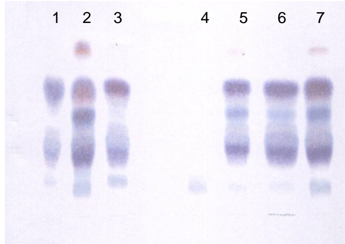
Supplementary Fig. S1. Analysis of diaminopimelic acid (DAP) isomers in strains 3-M5-R4 T and 3-M5-R7 and related strains. Lanes: 1, T. duodecadis ATCC 13347 T ; 2, T. japonica DSM 13192 T ; 3, 3-M5-R4 T ; 4, DAP standard; 5, T. australiensis DSM 12890 T ; 6, 3-M5-R7; 7, Bacillus lehensis MTCC7633 T .
