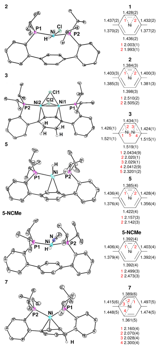
Fig. 1. Solid-state structures of 2 , 3 , 5-OTf , 5-NCMe-OTf , 7-BAr F 24 (left) and selected C–C and Ni–C distances, including 1 (right). Solvent molecules, anions, and select hydrogen atoms have been cropped for clarity.
