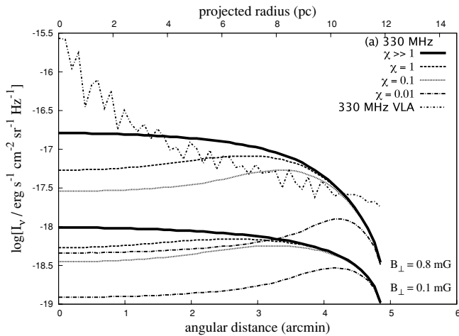
Figure 4. Comparison of the actual emission intensity as a function of angular distance from the center of Sgr B2 and that expected from models of synchrotron emission from secondary electrons at 330 MHz. The curves are for the parameters labeled and match those of Figure 9 of Protheroe et al. (2008).
