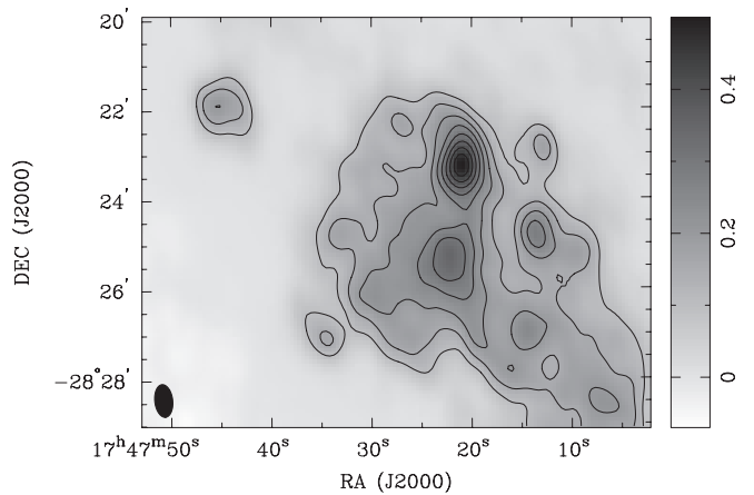
Figure 2. 330 MHz total intensity medium resolution image of Sgr B2 with a beam of 43'' × 24'' (located in the lower left corner; LaRosa et al. 2000). The contours are 330 MHz total intensity contours at 0.1, 0.15, 0.2, 0.25, 0.3, 0.35, 0.4, and 0.45 Jy beam -1 . The intensity scale on the right is in units of Jy beam -1 and is set from -0.07 to 0.5 Jy.
