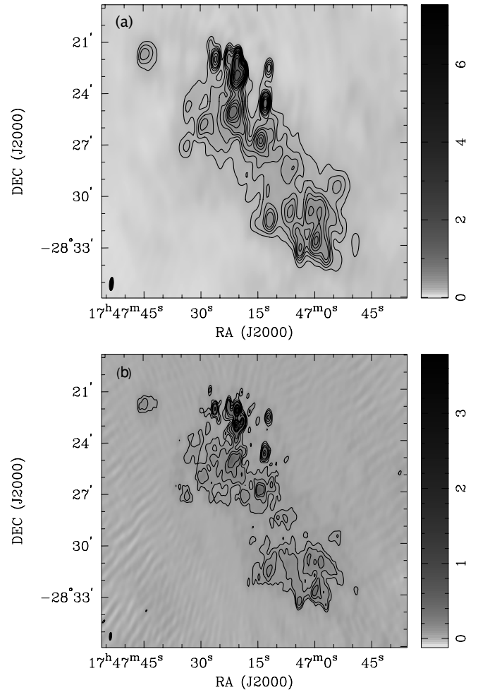
Figure 3. Close-up of the Sgr B region at (a) 1384 MHz and (b) 2368 MHz. The 1384 MHz image has contours at: 0.2, 0.25, 0.3, 0.35, 0.4, 0.5, 0.6, 0.7, 0.8, 1.0, 1.2, and 1.4 \text{Jy beam}^{-1} and a resolution of 47'' \times 14'' with the beam located in the lower left-hand corner. The 2368 MHz image has contours at: 0.08, 0.12, 0.2, 0.3, 0.64, 0.8, 1.0, 1.2, 1.5, and 1.8 \text{Jy beam}^{-1} and a resolution of 27'' \times 8'' with the beam located in the lower left-hand corner. The rms noise level of the images are 10 \text{ mJy beam}^{-1} at 1384 MHz and 5 \text{ mJy beam}^{-1} at 2368 MHz, matching the sensitivity at 1384 MHz of similar-resolution images.
