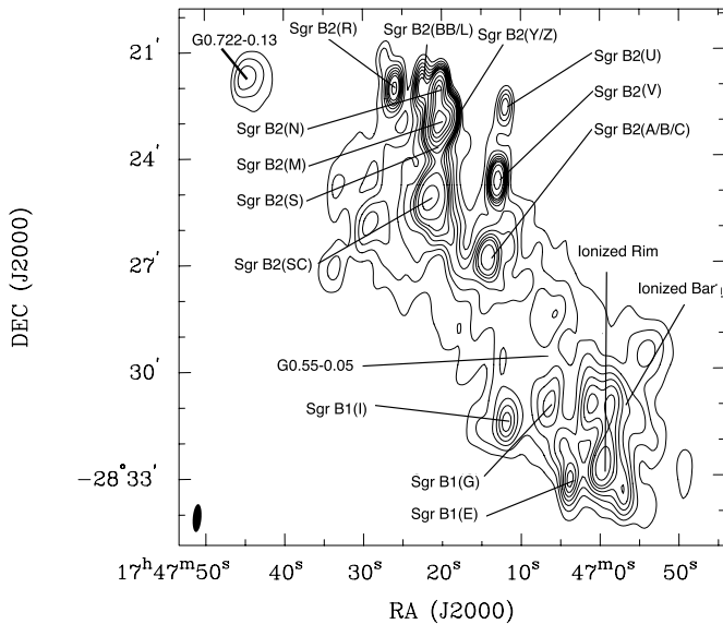
Figure 1. Image of 1384 MHz total intensity contours of the Sgr B region showing the sources as labeled in Table 2. Contours are at 200, 250, 300, 350, 400, 450, 500, 600, 800, 1000, and 1600 mJy beam -1 . The image has a resolution of 47'' × 14'', which is illustrated by the beam in the lower left-hand corner.
