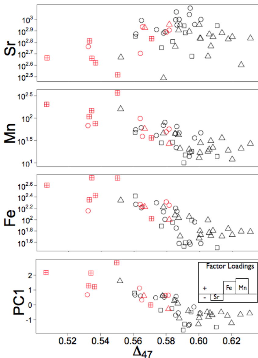
Figure S7 Trace element concentration (in ppm) plotted against \Delta_{47} for Sr, Mn, and Fe, (panels 1-3) and the first principal component (PC1) of log-transformed Sr, Mn, and Fe concentration (panel 4) for all 51 skeletal carbonate samples for which trace metal concentrations were measured. Inset in panel for shows relative factor loadings for PC1, which accounts 86% of variance in trace metal concentrations. Symbols as in main text figure 2; red symbols are those with clear textural alteration.
