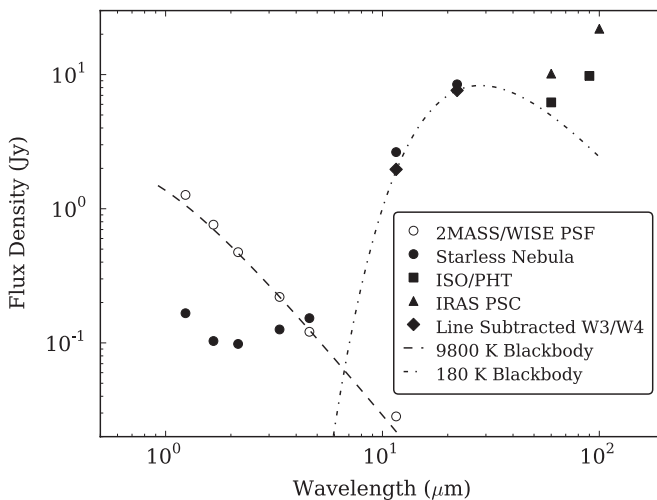
Figure 5. Plot of the integrated nebula SED using the dereddened 2MASS, WISE, ISO / PHT , and IRAS fluxes. The central source flux (found by point-spread function fitting) is shown for comparison and is represented by the open circles, the integrated nebular flux (see the text) is given by the filled circles, and the ISO and IRAS point source fluxes are indicated by the filled squares and triangles. An estimate of the contribution of the atomic lines was subtracted from the W3 and W4 fluxes, and this net thermal emission is indicated by the filled diamonds. A 9800 K blackbody curve is overlaid on the CSPN fluxes while a 180 K blackbody is drawn through the WISE line-corrected W3 and W4 fluxes to suggest that the character of the mid-infrared nebular emission is thermal in nature.
