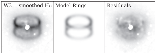
Figure 9. Residuals of the ring model fit for the W3 image. A smoothed version of the H\alpha image has been subtracted to remove the inner shell from the W3 image (left panel); this image was then rotated clockwise 131^\circ so the polar axis is vertical. The ring model (center) was then subtracted to reveal the residuals (right). While not a perfect fit due to the oversimplicity of the model, the general orientation and aspect ratios seem to be correct.
