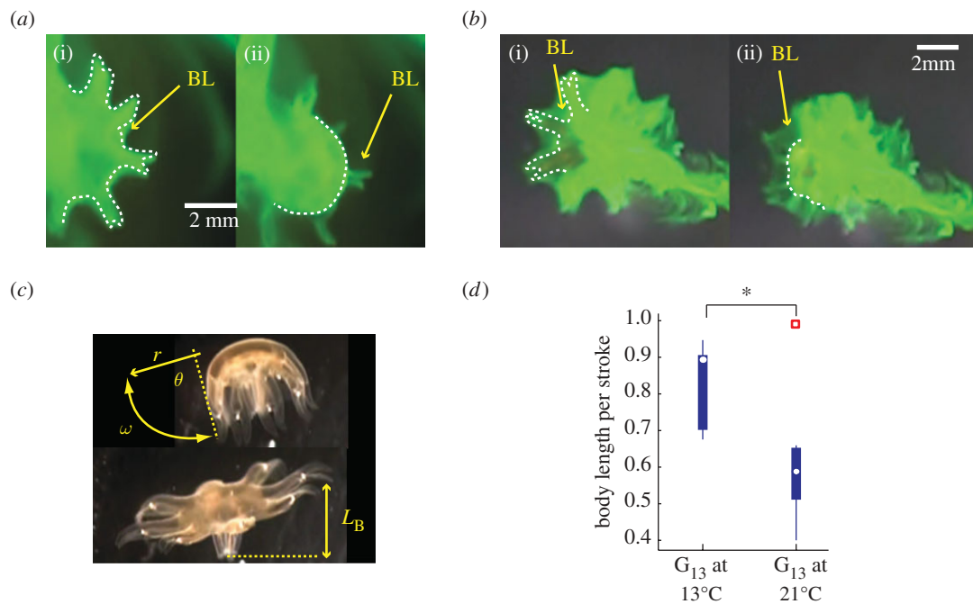
Figure 2. Dye visualization of boundary layer during powerstroke. Dotted line indicates outline of animal body. BL, boundary layer. (a) Sieve-mode: G_{13} ephyra swimming at 21^{\circ}\text{C} water temperature. (i) Start of powerstroke, bell is fully relaxed, (ii) end of powerstroke, bell is fully contracted. Note that the thin boundary layer outlines the body but fails to connect between lappets. (b) Paddle-mode: G_{13} ephyra swimming at 13^{\circ}\text{C} water temperature. (i) Start of powerstroke, bell is fully relaxed, (ii) end of powerstroke, bell is fully contracted. Note the delay in boundary layer motion when compared with body motion, visualizing the velocity gradient at the fluid–solid interface. (c) Parameters of ephyra propulsion. r , Radial position along lappet; \theta , swept angle; \omega , angular velocity; L_B , body length. (d) Effect of ambient water temperature on propulsion efficiency of G_{13} ephyrae. Box plots show body length travelled per stroke at 13^{\circ}\text{C} ( n = 7 ) and at 21^{\circ}\text{C} ( n = 7 ). White marks correspond to median, the edges of the box are 25th and 75th percentiles, whiskers indicate extreme data points not considered outliers. Outliers are plotted as individual squares. Asterisk represents significant difference in median values.
