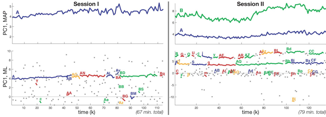
Fig. 3. Graphical comparison of the tracking ability of the MAP versus ML algorithms in two sessions, each lasting over an hour. Each plot depicts the first principal component of the cluster means versus time. Neuron tracks are represented by lines and labeled by letter ID. Gray dots indicate a neuron ID lasting only one time step (for which the letter label is suppressed). Note that the MAP algorithm (upper graphs) produces unbroken tracks with single IDs, whereas the ML algorithm (lower graphs) clusters the data inconsistently, losing the tracks frequently, and generating many spurious clusters.
