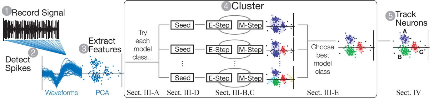
Fig. 1. Structure of the algorithm. Before clustering takes place: 1) the electrode signal is recorded for a brief sampling interval; 2) neuronal spike waveforms are detected in this voltage trace and aligned by their minimum; and 3) spikes are projected onto an appropriate feature space, such as a 2-D PCA basis. 4) Next, these data points are clustered using EM optimization of a GMM, over several possible model classes. 5) Finally, neurons are tracked by associating the clusters from the current interval to the previous interval. This entire process is repeated for every sampling interval.
