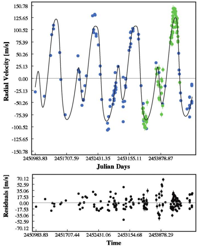
FIG. 2.—Best-fit integrated solution to the RV data presented in this article (blue) and the HET data (green) reported by Wittenmyer et al. (2009; orbital parameters listed as Fit B in Table 3).
