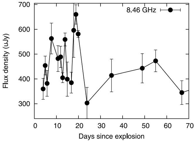
FIG. 3.—Long-term light curve at 8.46 GHz showing evidence of ISS. This scintillation is refractive in nature and starts dominating once diffractive scintillation quenches (see text for more details).
