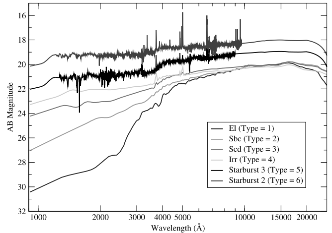
FIG. 1.—Spectral energy distributions from Mobasher et al. (2007) used to compute COSMOS galaxy spectral types and photometric redshifts. This figure is a reproduction of Fig. 1 of Mobasher et al. [See the electronic edition of the Journal for a color version of this figure.]
