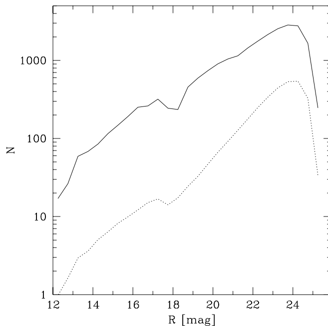
FIG. 22.—Magnitude distribution of possible counterparts ( solid curve ) and background objects ( dotted curve ) within a 2'' radius from each 24\ \mu\text{m} source. The solid curve has been normalized according to eq. (10) and used in the likelihood ratio definition.
