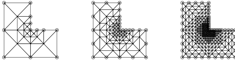
FIG. 3. Example 2: Nested finite element meshes for MG.
