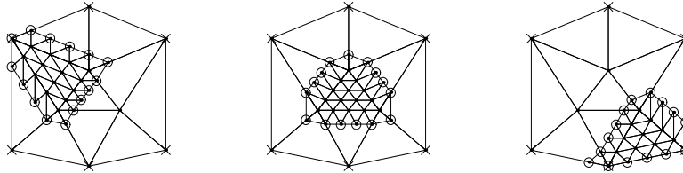
FIG. 2. Example 1: Overlapping subdomains for DD.
