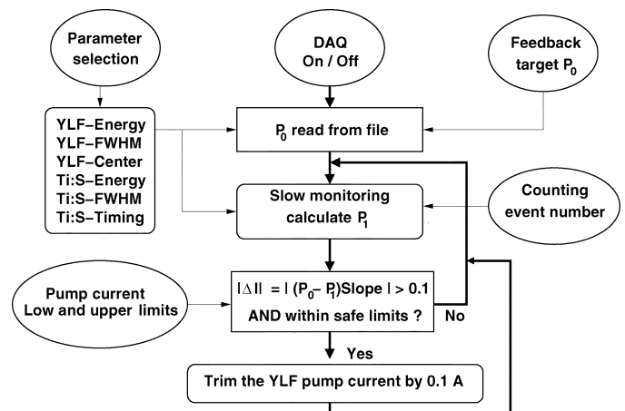
Fig. 7. A schematic describing the software feedback control.
