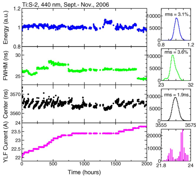
Fig. 11. The same as Fig. 9 for combined Ti:Sapphire laser runs at 440 nm for more than 3 months.
