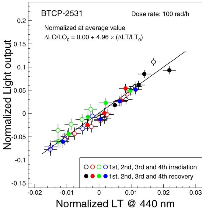
Fig. 2. The normalized variations of the light output are shown as a function of the normalized variations of the longitudinal transmission at 440 nm for sample BTCP-2531 under 100 rad/h irradiation.
