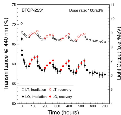
Fig. 1. Variations of the longitudinal transmission (left scale, open circles) and the light output (right scale, solid dots) are shown as a function of time for a full size CMS PbWO 4 crystal BTCP-2531 in a multi-cycle irradiations of 100 rad/h followed by recoveries.
