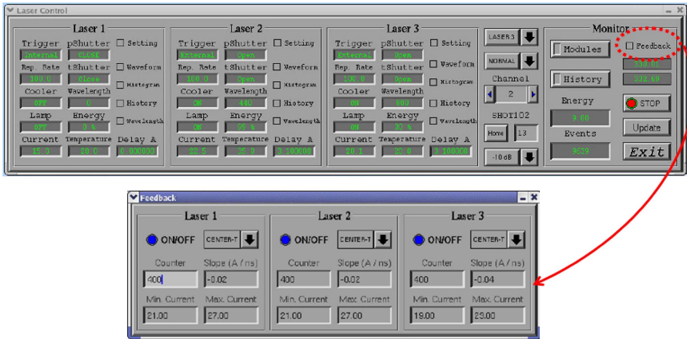
Fig. 8. The graphic interface of the laser DAQ control panel (top) and the feedback setting window (bottom).
