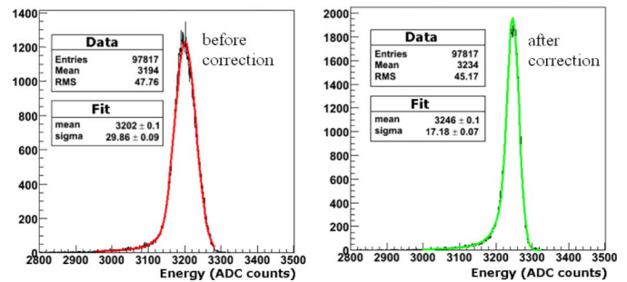
Fig. 13. The energy resolutions of 120 GeV electrons, reconstructed by summing 3 \times 3 crystals in an irradiation study, are shown before (left) and after (right) the monitoring corrections.
