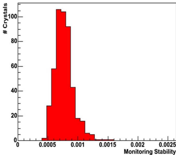
Fig. 12. The monitoring system stability shows a 0.1% is achieved in the ECAL beam test.
