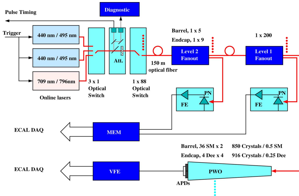
Fig. 3. A schematic showing the CMS laser monitoring system.
