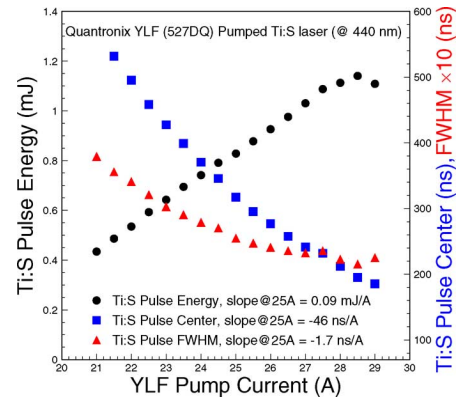
Fig. 6. Correlations between the Nd:YLF laser pumping current and the Ti:Sapphire laser pulse energy, width (FWHM) and the pulse center timing.
