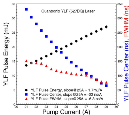
Fig. 5. Correlations between the Nd:YLF laser pumping current and the Nd:YLF laser pulse energy, width (FWHM) and pulse center timing.
