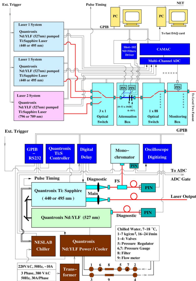
Fig. 4. A schematic (top) showing the design of the laser light source and the high level distribution system (LSDS) with the details of one laser system shown at the bottom.
