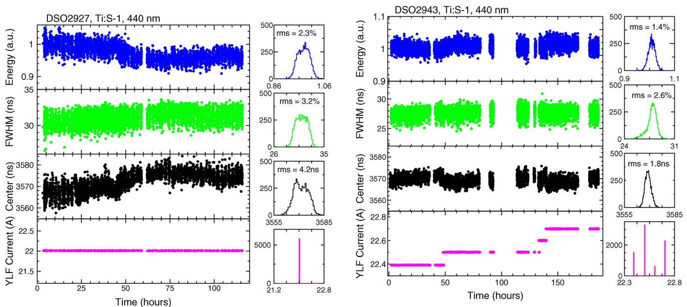
Fig. 10. The same as Fig. 9 for a Ti:Sapphire laser run at 440 nm for more than 180 hours by using the Ti:Sapphire laser pulse timing as the software feedback parameter.
