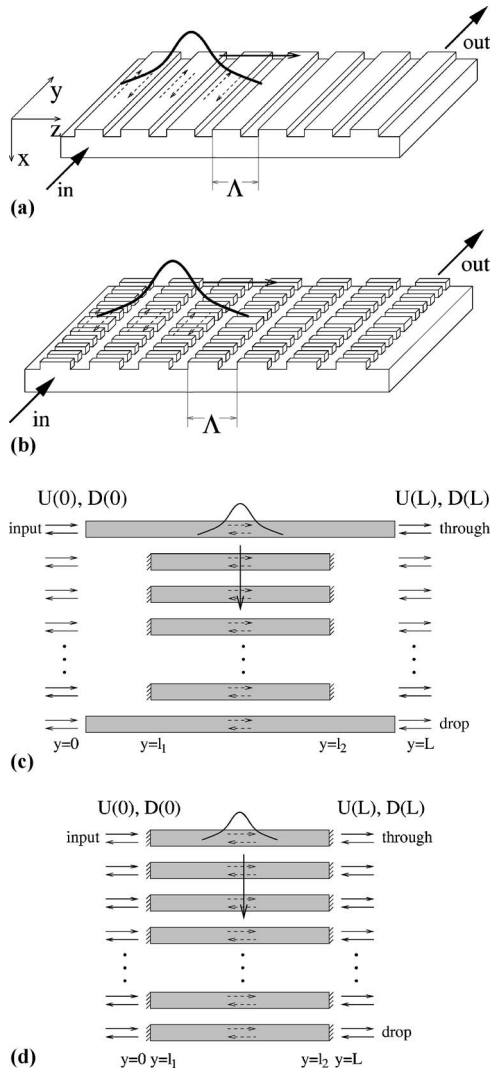
Fig. 1. Schematic of (a) waveguide laser and (b) DFB laser arrays in a planar geometry as implementations of CROWs. The input–output can be (c) side coupled or (d) end coupled into–out of the array. \Lambda is the period of the CROW. The slanted lines represent reflectors that define each resonator. The arrows indicate the field propagation direction inside each resonator or waveguide. An optical pulse in the structure propagates in the direction of periodicity of the resonators.
