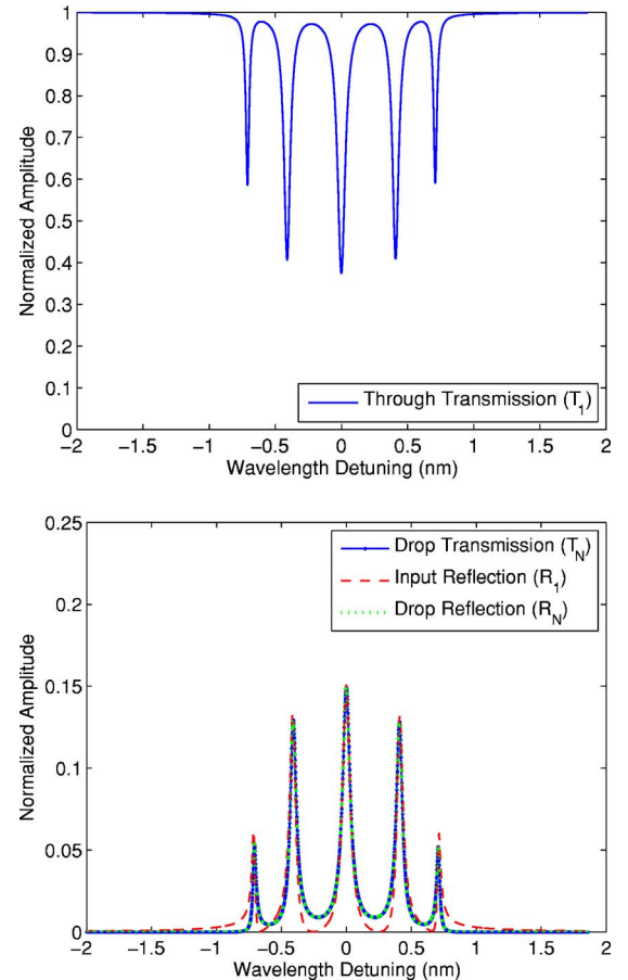
Fig. 3. (Color online) (a) Transmission spectrum at the through port and (b) the transmission and reflection spectra at the input and drop ports for the side-coupled array.
