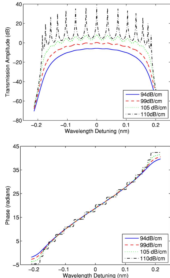
Fig. 4. (Color online) (a) Transmission and (b) phase responses of a resonator array for various gain values. The input is end coupled into the first element of the array.
