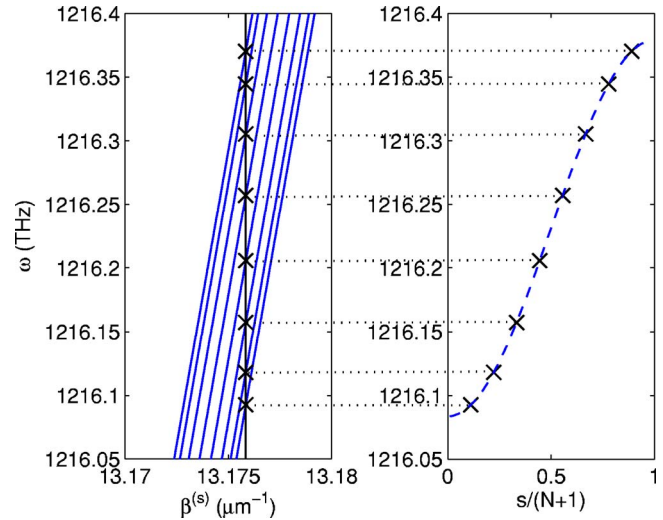
Fig. 2. (Color online) Schematic illustrating the role of the additional resonance or boundary condition in y . On the left, the resonance condition \beta^{(s)}L = m\pi selects the resonance frequencies from the dispersion relations of the waveguide array. These frequencies correspond to particular values of s\pi/(N+1) on the right.
