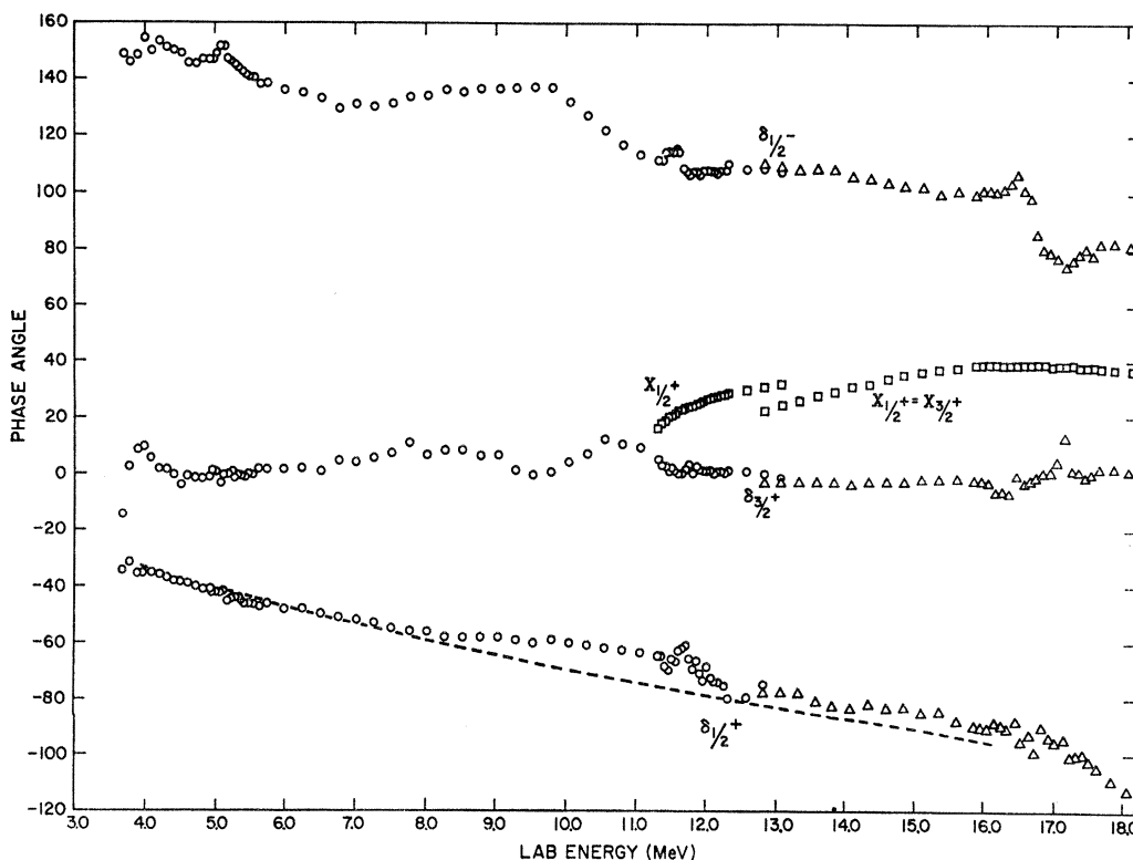
FIG. 15. H^3(\alpha, \alpha)H^3 phase shifts in degrees showing the phase shifts \delta_{1/2}^+ , \delta_{1/2}^- , and \delta_{3/2}^+ as a function of energy. Also shown are the parameters X_{1/2}^+ and X_{3/2}^+ . The dashed line is a fit to the phase shift \delta_{1/2}^+ and corresponds to the s -wave scattering from a hard sphere of radius 2.6 F. The change of symbols near 13 MeV indicates that the phase shifts and X_{J\pi} 's obtained above this energy used the negative ion injection-beam data. Below this energy, the neutral injection-beam data were used.
