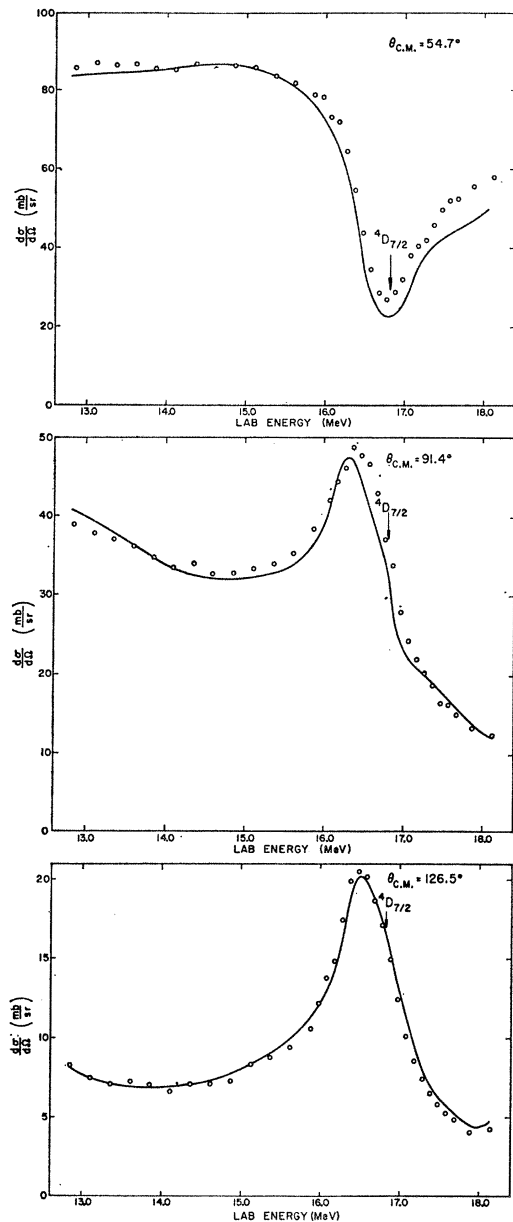
FIG. 5. Three typical excitation curves from the \text{H}^3(\alpha, \alpha)\text{H}^8 experiment above 12.8 MeV. Symbols are the same as in Fig. 3.
