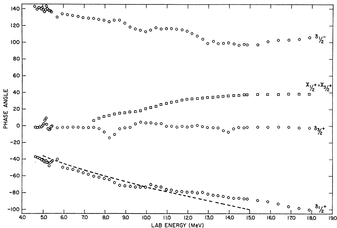
FIG. 11. He 4 (He 3 ,He 3 )He 4 phase shifts in degrees showing the phase shifts \delta_{1/2}^+ , \delta_{1/2}^- , and \delta_{3/2}^+ as a function of energy. Also shown are the parameters X_{1/2}^+ and X_{3/2}^+ . The dashed line is a fit to the phase shift \delta_{1/2}^+ and corresponds to the s -wave scattering from a hard sphere of radius 2.8 F.
