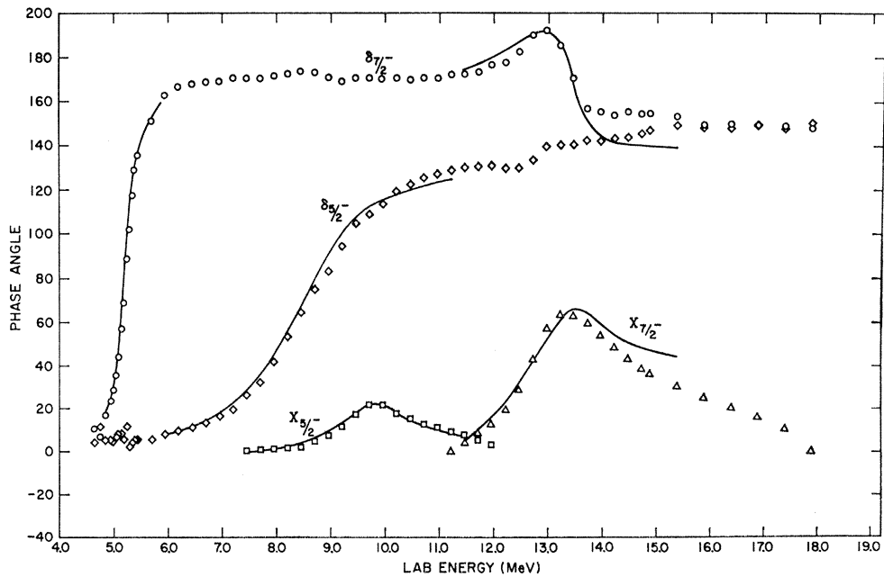
FIG. 13. \text{He}^4(\text{He}^3, \text{He}^3)\text{He}^4 phase shifts in degrees showing the phase shifts \delta_{7/2}^- and \delta_{5/2}^- . Also shown are the parameters X_{7/2}^- and X_{5/2}^- . The lines show the fits to the phase shifts from R -matrix theory.
