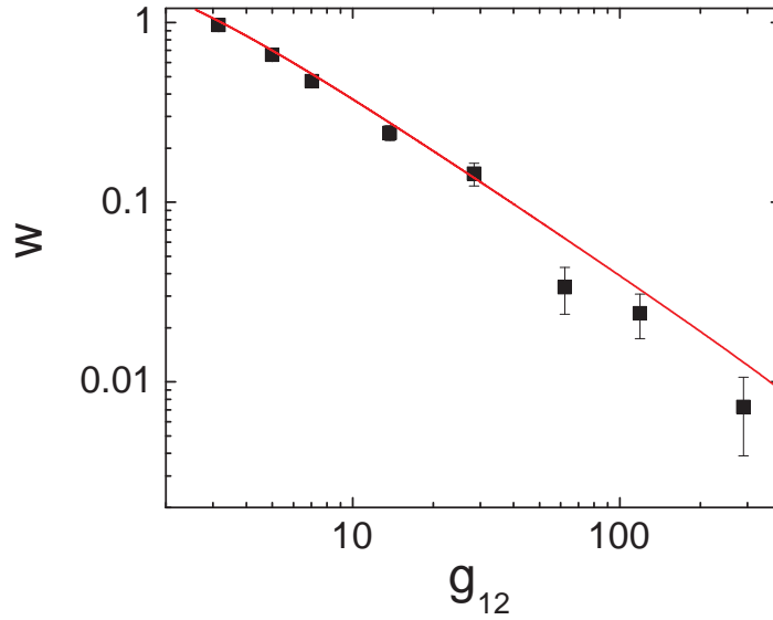
Fig. 3. Suppression of the two-photon component of field 2 conditioned on the detection events in field 1, measured by the w parameter, as a function of g_{12} . The lowest value obtained is 0.007 \pm 0.003 . All points in this plot were obtained without trapping light between trials. The full curve is from a fit based on the simplified model of Ref. [15], with the same parameters as in Fig. 2.
