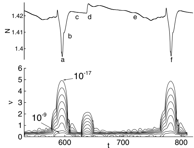
FIG. 2. Time series N(t) (top) and corresponding spectrogram (bottom) for one period of case (ii). The labels a-f represent particular moments in the evolution of the pattern and are discussed in the text. The spectrogram displays 9 orders of magnitude of the power, P(\nu) , with the smallest and largest contours labeled; the remaining contours each differ by a factor of 10. The spectrogram was calculated using a sliding Hann window of width \Delta t = 20.48 and linearly detrended overlapping segments (segments overlap by t = 20.0 ).
