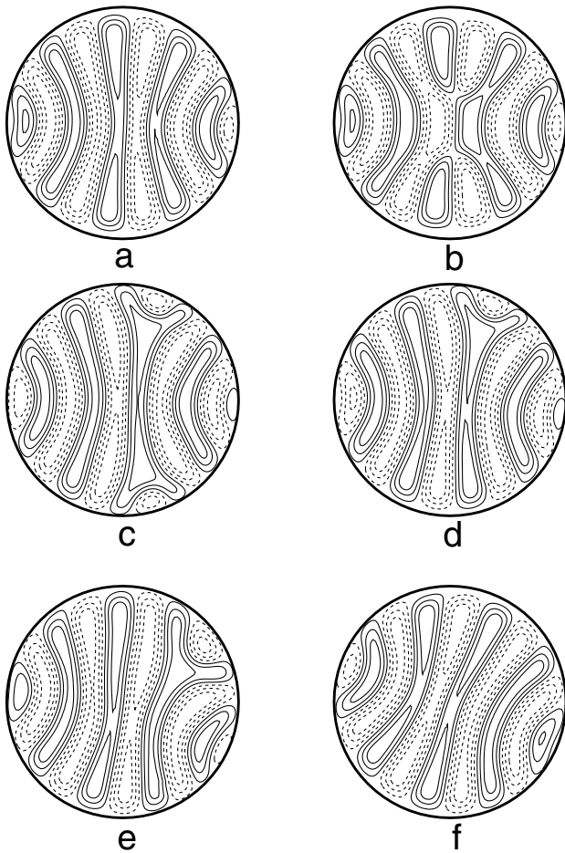
FIG. 6. Flow visualization showing contours of the thermal perturbation at the mid-depth, (six evenly spaced contours; -0.2 \leq \delta T \leq 0.2 , negative values are dashed lines, and positive values are solid lines) for case (ii). Panels (a)–(f) are for t = 600, 605, 630, 650, 735, 785 . The dislocations glide to the right; during the next period, the dislocations glide to the left, as can already be discerned in (f) by the bias in the roll compression. This left and right alternation continues for the entire simulation.
