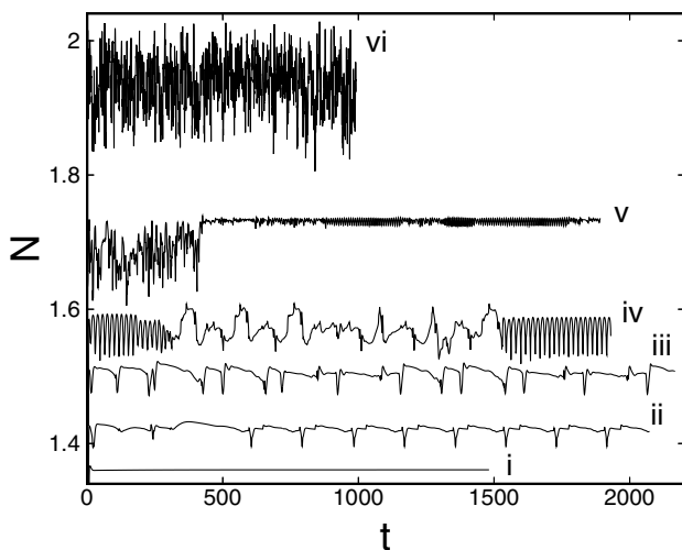
FIG. 1. Plots of the dimensionless heat transport N(t) for cases (i-vi) for reduced Rayleigh number \epsilon = 0.557, 0.614, 0.8, 1.0, 1.5, and 3.0 , respectively. For cases (i-v), \Delta t = 0.01 , and for case (vi), \Delta t = 0.005 ( \Delta t is the time step).
