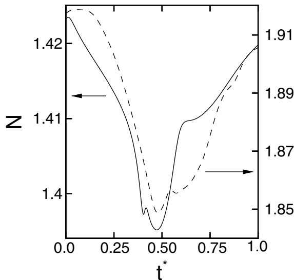
FIG. 4. A closeup of the time series N(t) , illustrating the signature of a nucleation of a dislocation pair for case (ii) (solid line), and the signature of a roll pinch-off for case (vi) (dashed line). Time t^* is measured as t^* = (t - t_i)/\Delta t ; t_i denotes when the event begins, and \Delta t is the duration of the event. For the events shown, t_i = 587, 270.5 and \Delta t = 18, 1.5 for cases (ii) and (vi), respectively.
