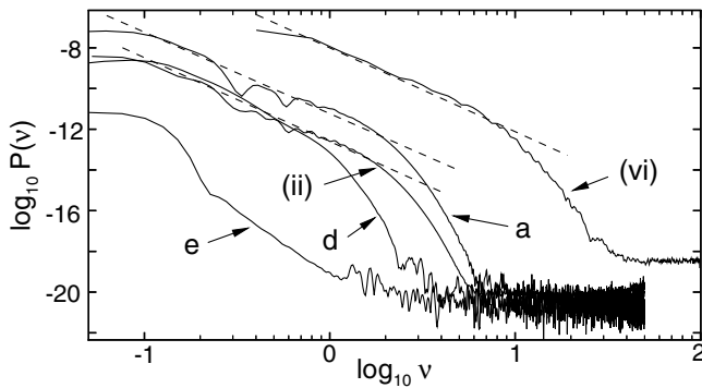
FIG. 3. Windowed power spectra. The power spectra labeled (a), (d), and (e) are vertical slices of the spectrogram taken at representative times for case (ii) at dislocation nucleation, dislocation annihilation, and dislocation glide, respectively. The curves labeled (ii) and (vi) are the average of the windowed power spectra using the entire spectrogram for cases (ii) and (vi). The dashed lines represent P(\nu) \sim \nu^{-4} .
