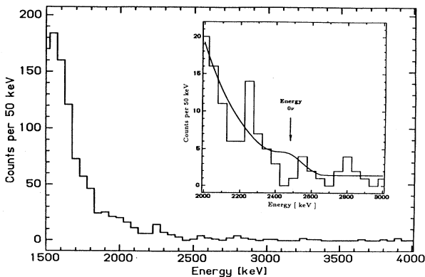
FIG. 9. Energy spectrum of two-electron candidate events, from 6830 h of data. The 90% C.L. limit for a hypothetical 0\nu peak at 2481 keV is represented by the solid line in the inset.
