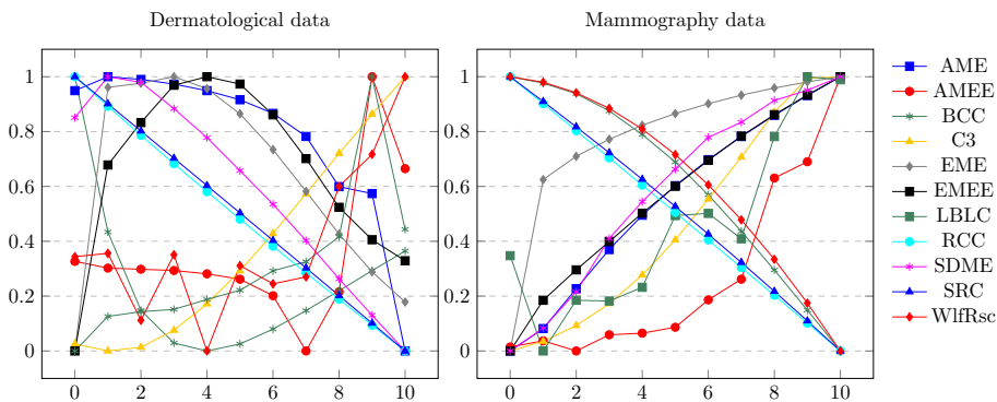
Fig. 3. The measures behaviour for the Gaussian noise image degradation. Left: dermatological data (colour), right: mammography data (grayscale).
