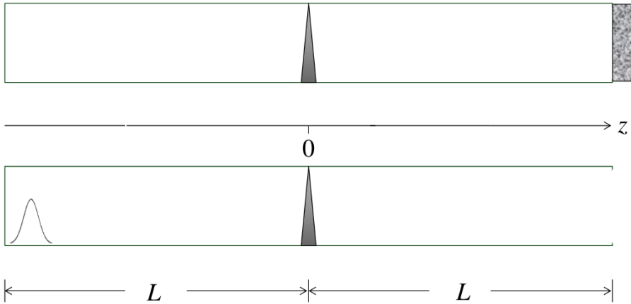
Figure 3. Two parallel cavities, with a single neutron wave packet (here in the lower cavity) and a single mirror (closing the upper cavity).
