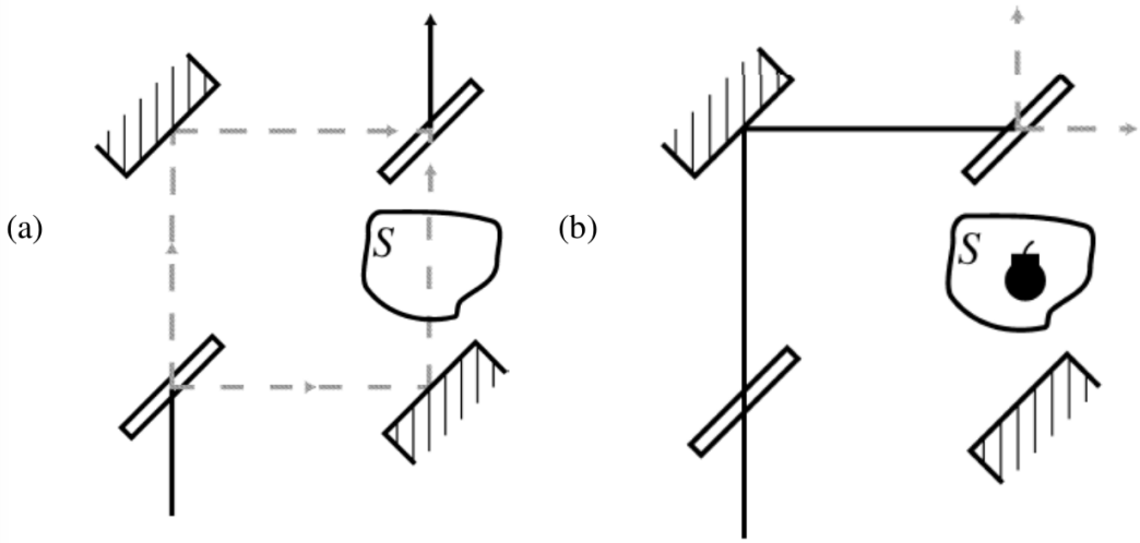
Figure 1. The Elitzur-Vaidman interaction-free measurement. (a) With a well defined relative phase between the arms, photons exit the interferometer in one direction only. (b) A bomb, by not exploding, provides which-path information.
