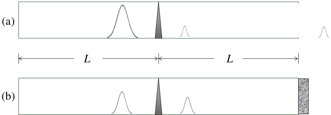
Figure 4. (a) A term in the post-selected state \Psi_{fm}(z, Z, T) of Eq. (5). Since no mirror is present to reflect the neutron from the right end of the cavity, the wave packets to the right of the partition have amplitudes of order \epsilon and move away from the partition. (In the time-reversed account, they approach the partition.) (b) A term in the evolution of the pre-selected state \Psi_{in}(z, Z, 0) of Eq. (4). The mirror reflects the neutron which, over a time T , passes completely through the partition.
