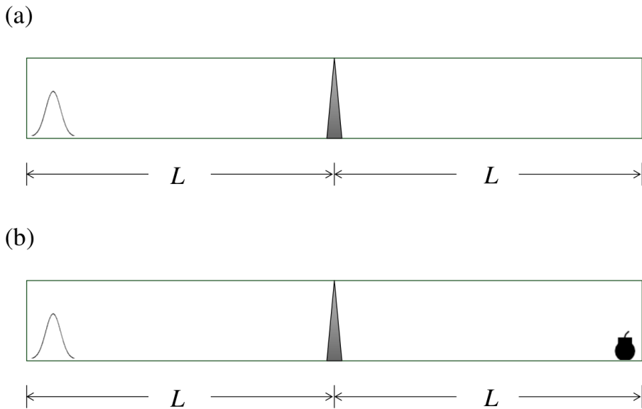
Figure 2. One-dimensional cavity of length 2L with a partition at its center, (a) without and (b) with a bomb at the right end.
