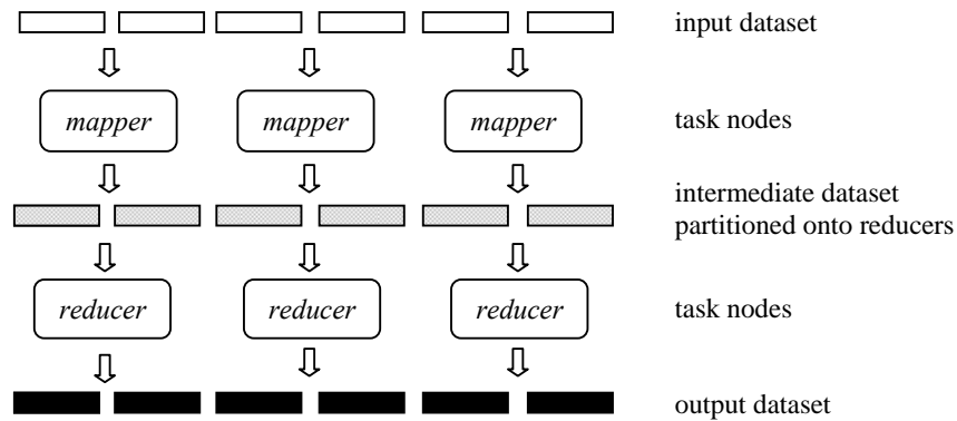
Fig. 1. A simplified representation of an MR job. The size of the output dataset can be different from the size of the input data set. An MR cluster consists of a number of tasks nodes and a single main node that controls tasks nodes. All mappers and reducers run on task nodes.
