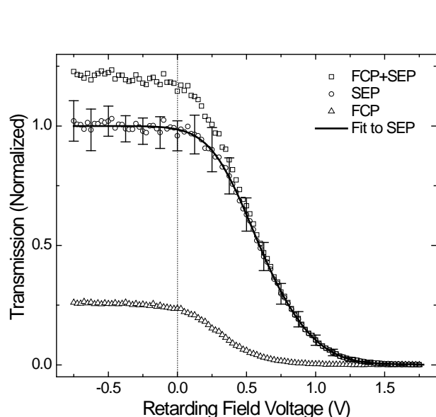
Figure 1. Transmission of vibrationally promoted exoelectrons as function of retarding potential. See text.
