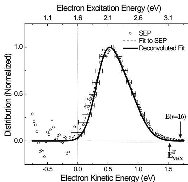
Figure 2. Kinetic energy distribution of vibrationally promoted exoelectrons derived from the data in Figure 1. See text.
