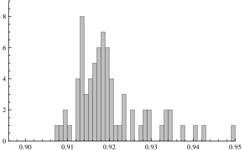
FIG. 4. Histogram of the magnitudes of the curvature corrections to the first 72 knot and link lengths.
