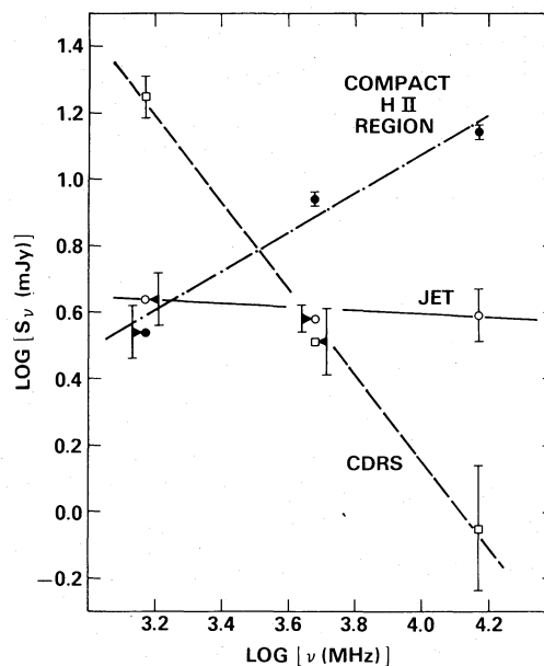
FIG. 3.—Shown are the regression lines which determine the spectral indices of the CDRS, the compact H II region around the hot companion, and the jet \sim 6'' northeast of the LPV. Actual values of the spectral indices are presented in Table 1.
