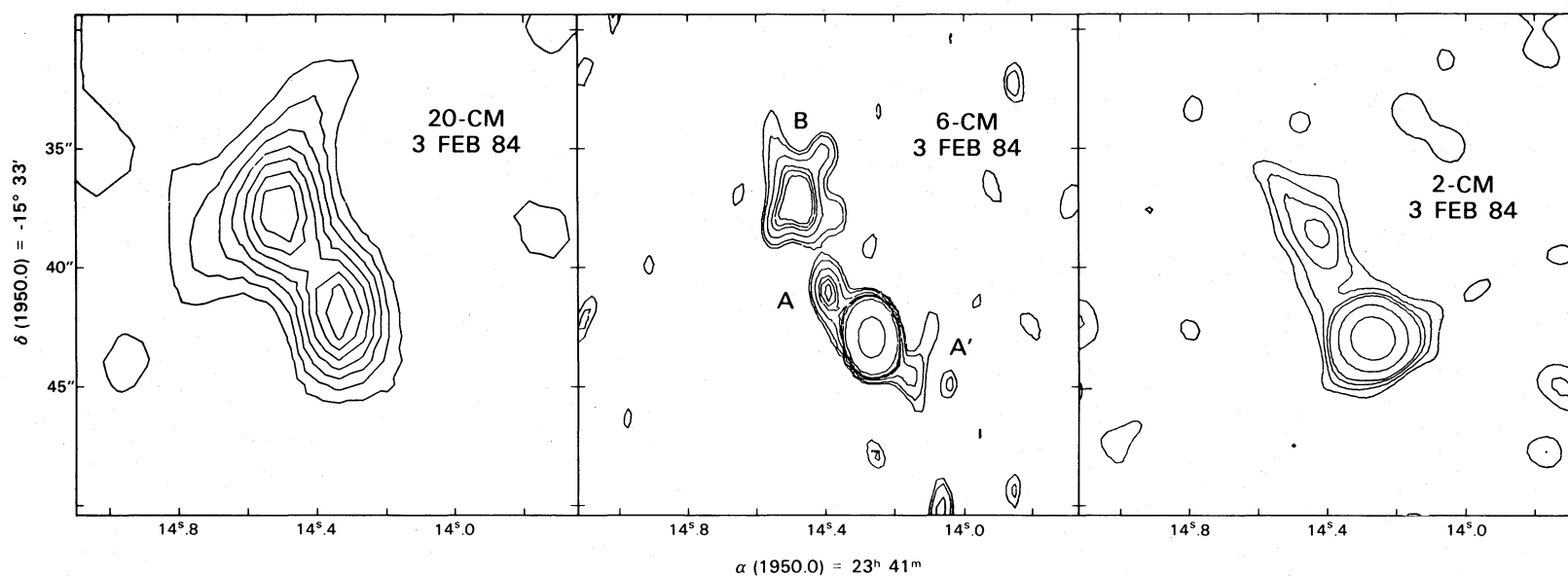
FIG. 1.—(left) This 20 cm map shows the jet rivals the compact H II region with regard to both peak and integrated flux (see Table 1) at this wavelength. Contour levels are 0.5, 0.8, 1.1, 1.4, 1.7, 2.0, and 2.3 mJy; peak fluxes for both blended features are each \sim 2.7 mJy per beam. The 1.4 contour level shows the approximate beam shape. (middle) This 6 cm map shows all the radio features so far detected in the immediate vicinity of R Aquarii. Contour levels are 0.15, 0.20, 0.30, 0.40, 0.45, 0.50, 0.75, and 3.70 mJy; peak flux for the compact H II region in this map is \sim 7.3 mJy per beam. The 3.7 contour level shows the approximate beam shape. (right) This 2 cm map clearly shows the jet at this wavelength for the first time. Contour levels are 0.35, 0.60, 0.85, 1.10, 2.50, and 6.20 mJy; peak flux for the compact H II region is \sim 12.4 mJy per beam. The 6.2 contour level shows the approximate beam shape.
