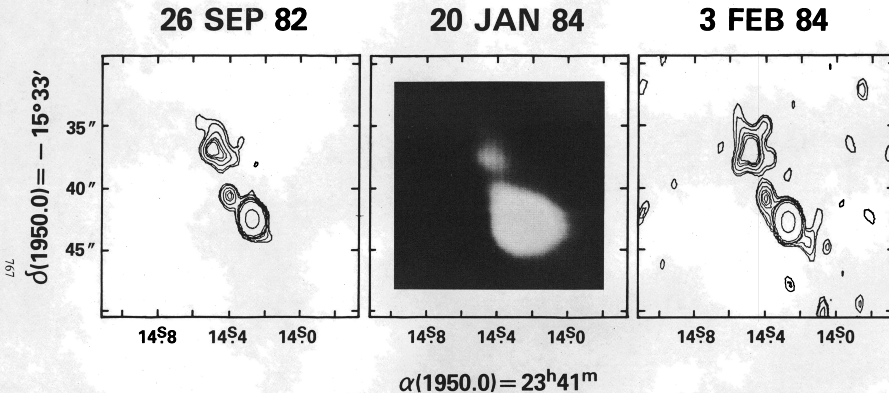
FIG. 2.—(left) This 6 cm has the same contour levels as the middle panel of Fig. 1 except these data have a peak flux of \sim 7.5 mJy per beam. We used a subset of these data to mimic the parallactic angle coverage of the data shown in the right panel of this figure; this resulted in a greater morphological similarity between the 1984 and 1982 radio data sets. However, the full data set shown here more accurately depicts the true structure as shown in the optical data of the middle panel. (middle) This optical photograph of R Aquarii is predominantly in the light of H\beta at 4860 \text{ \AA} and H\alpha at 6563 \text{ \AA} ; the LPV is overexposed and the instrument suffers saturation on the LPV only. The similarity between the radio and optical data is remarkable as shown here; thus, this series of data indicate that the jet is now stable over time scales of a few years and argues for the jet's thermal nature at both optical and radio wavelengths. (right) This 6 cm map is a reproduction of Fig. 1 (middle panel) for ease of comparison with other data shown here. The apparent difference in the shape of the jet in this panel as compared to the leftmost panel is due to less complete parallactic angle coverage in the 1984 data set. However, these data more easily produce the weak feature (feature A' in Fig. 1) seen toward the southwest of the compact H II region than that seen in the 1982 data set; thus, we may be seeing a new feature evolving; it is interesting that this new feature is symmetrically placed with regard to the stronger feature toward the immediate northeast (feature A in Fig. 1).
