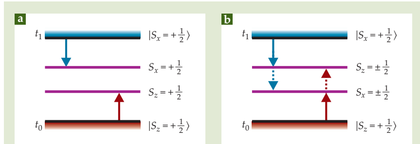
Figure 2. Measuring both the x and z spin components of a spin- 1/2 particle in the interval between the pre- and postselections of figure 1 yields different results depending on the time order of the two measurements. (a) If the first interim measurement is along the direction of the preselection and the second interim measurement is along the postselection direction, both measurements are determined by the selections. (b) Reversing the order of the interim measurements destroys that certainty.
