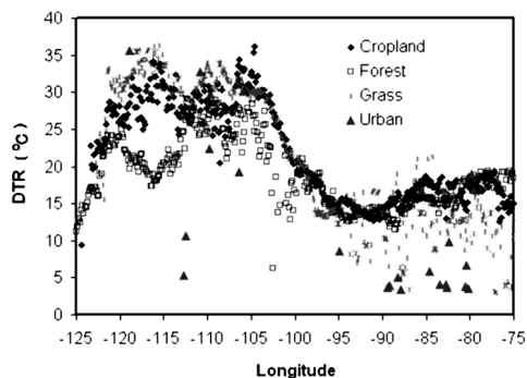
Figure 3. Meridional mean DTR derived from GOES-8 for cropland, forests, grassland and urban surfaces for a five-year average July.
