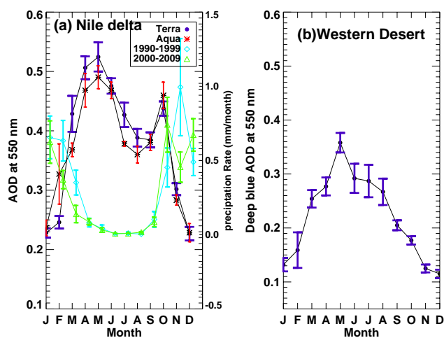
Fig. 3. (a) Climatology MODIS monthly AOD means over the Nile Delta from Terra (2000–2009) and Aqua (2003–2009), the right axis is for the precipitation rate of Nile Delta for 1990–1999 and 2000–2009. (b) Climatology MODIS monthly AOD means over the Western desert using Aqua deep blue (2003–2009) data product, the vertical bars represent the standard deviations.
