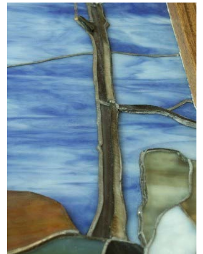
Figure 19: Tree, reverse side, before repair showing plated shading
