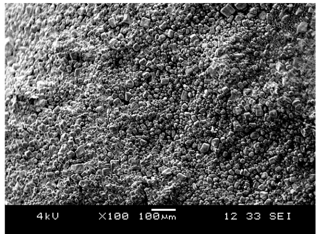
Figure 3-10 SEM of cross section of LTP pellets sintered at 1050 °C for 6 hours
