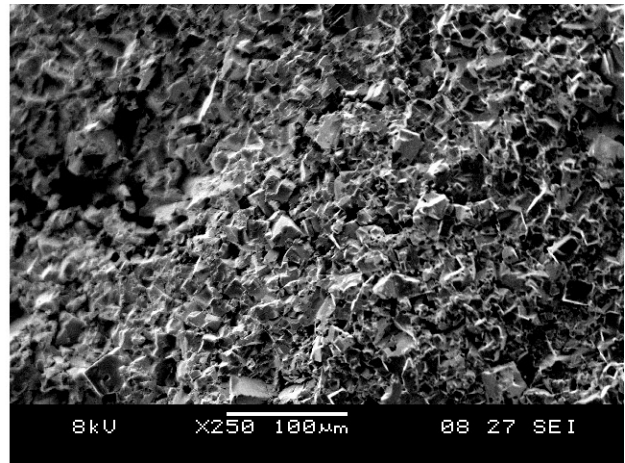
Figure 3-9 SEM of cross section of LTP pellets sintered at 950 °C for 6 hours
