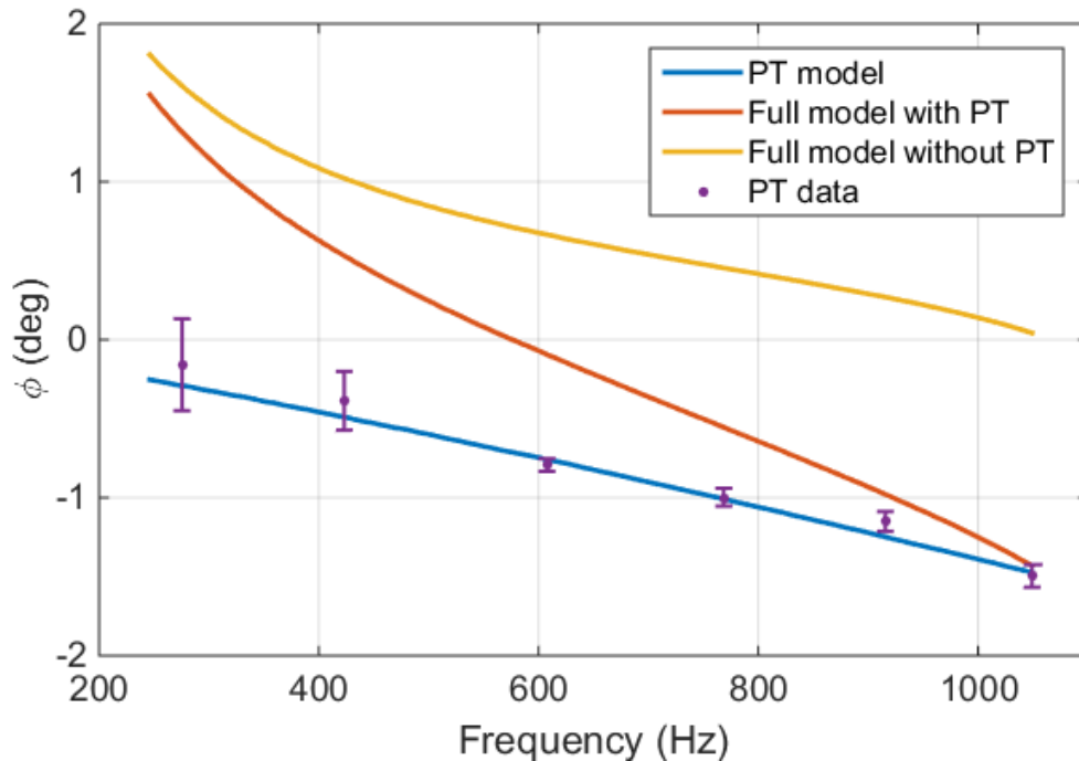
Figure 37 : Feedback phase in the system due to the optical spring and photo-thermal effect. The measured extra phase is consistent with 2.60 ppm of absorption. The error bars are as small as \pm 0.04^\circ , a remarkable precision for an open loop transfer function phase measurement.
