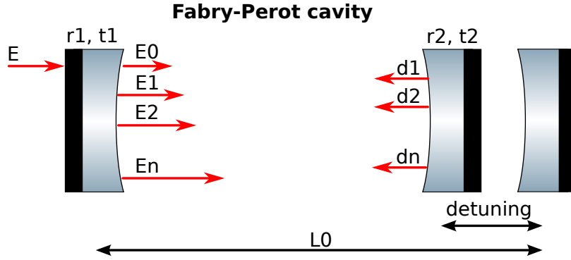
Figure 11 : A Fabry-Perot cavity of length L_0 and coefficients r_1, t_1 and r_2, t_2 for the input and end mirrors respectively. The input mirror is stationary while the end mirror is affected by harmonic motion. The incoming field E at each round-trip i adds up a phase shift due to the displacement d_i
