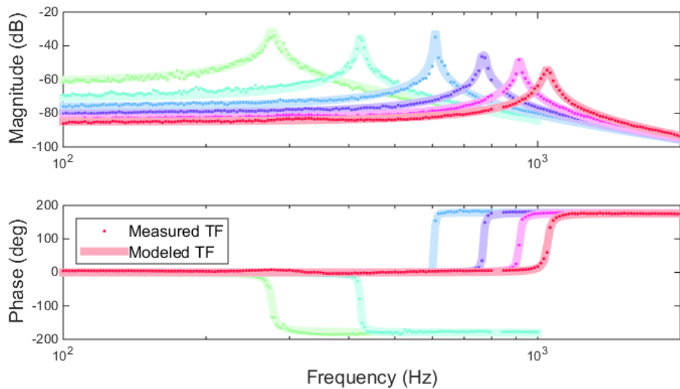
Figure 35 : Data and modeled transfer function for a series of stable and unstable springs. The modeled transfer functions include the full coating and spot size correction, computed with the measured average absorption. Stable springs show a phase drop of 180 degrees at resonance, while unstable springs show a rise of 180 degrees.
