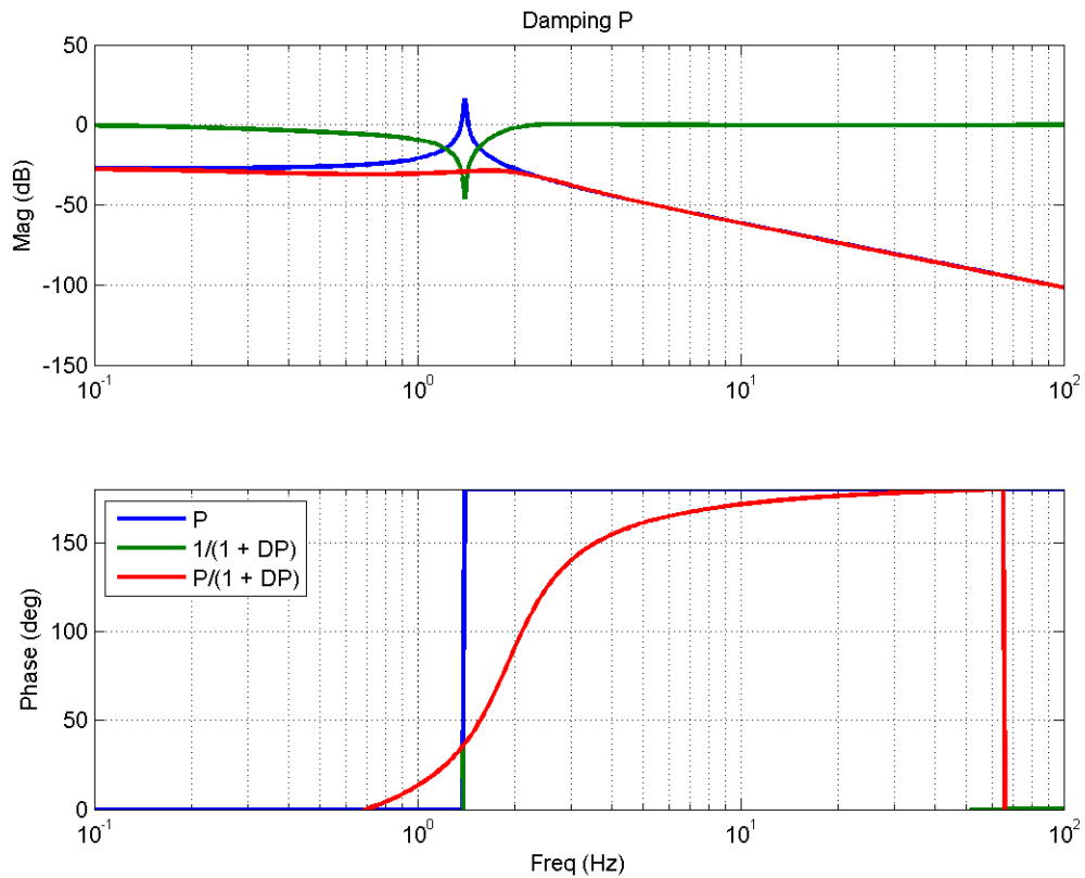
Figure 27 : Damped large mass pendulum transfer function.
