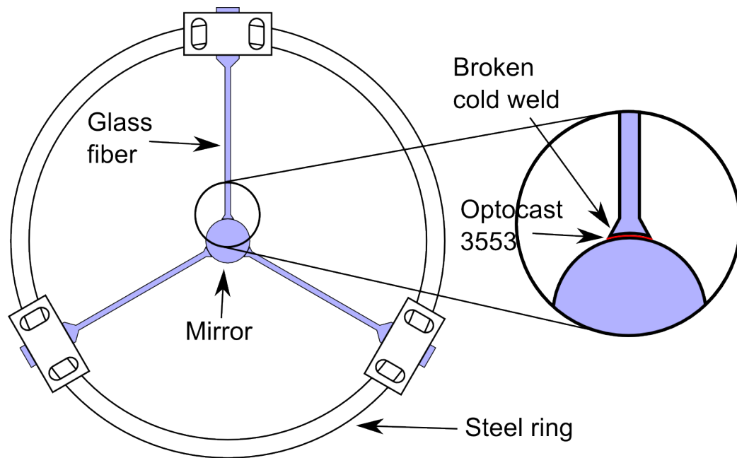
Figure 13 : End mass suspension. A 0.4 gram mirror is suspended from a steel ring using glass fibers. The nubs at the end of the fibers are glued onto the mirror using Optocast 3553. The rods on the other side of the fiber are glued into aluminum blocks which are tensioned then screwed down to the ring.
