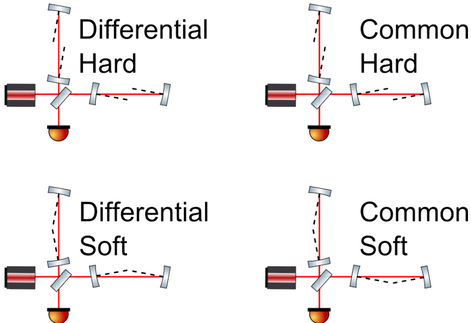
Figure 45 : The four Sides-sigg modes of the Fabry-Perot cavities in LIGO. The two hard modes are stable and the two soft modes are unstable. All of modes must be damped with control loops.
