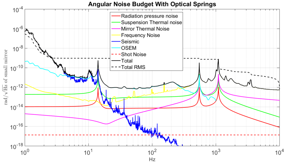
Figure 43 : Expected noise budget for the angular trap. The noises associated with mirror position motion or frequency noise are damped by an expected optical spring. At low frequencies, the total noise is dominated by seismic noise. Starting around 10 Hz, we see the effects of OSEM noise and laser frequency noise dominating the noise spectrum. At very high frequencies, we see the effects of thermal noise at the resonant frequencies of the optical springs.
