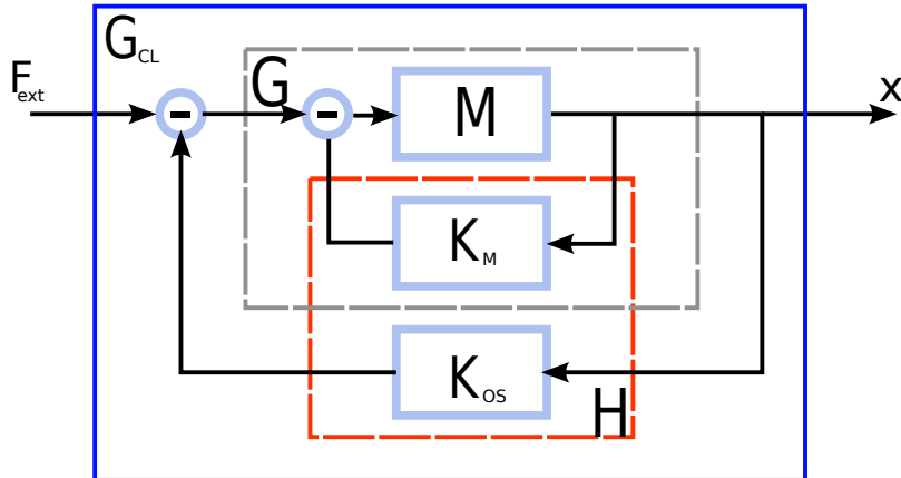
Figure 5 : Mechanical oscillator and feedback systems. The mechanical oscillator can be seen as plant ( G ) and the optical spring K_{OS} as feedback or alternatively as free test mass (plant M ) and H = K_{OS} + K_M as feedback. Both the cases lead to the same closed loop transfer function G_{CL} which describes the system as a damped mechanical oscillator in the presence of the optical spring, which is subjected to the external force F_{ext} and has the corresponding displacement x as output.
