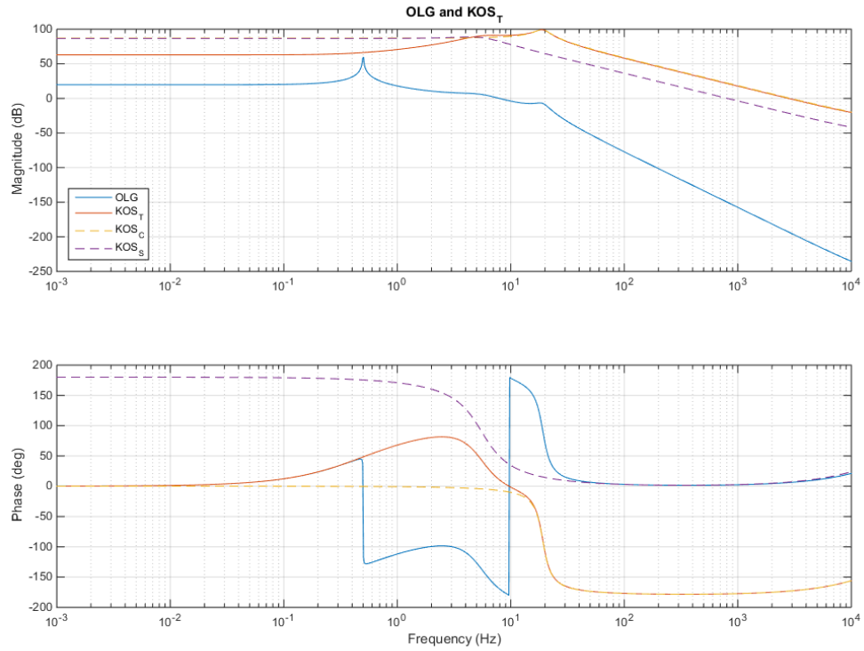
Figure 47 : Open loop gain ( OLG ) of the angular control scheme and optical springs. The optical springs shown are the carrier and subcarrier optical spring constants ( KOS_C and KOS_S ) and the total optical spring ( KOS_T ).
