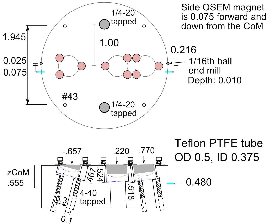
Figure 12 : The input coupler for the cavity. Three 0.5 inch diameter mirrors with 7.5 cm RoC are held at specific angles inside an aluminum disk. The two side mirrors are adjustable using set screws, while the central mirror is fixed. All of the mirrors have been shifted 0.2 inches in the positive direction to center them in the disk.
