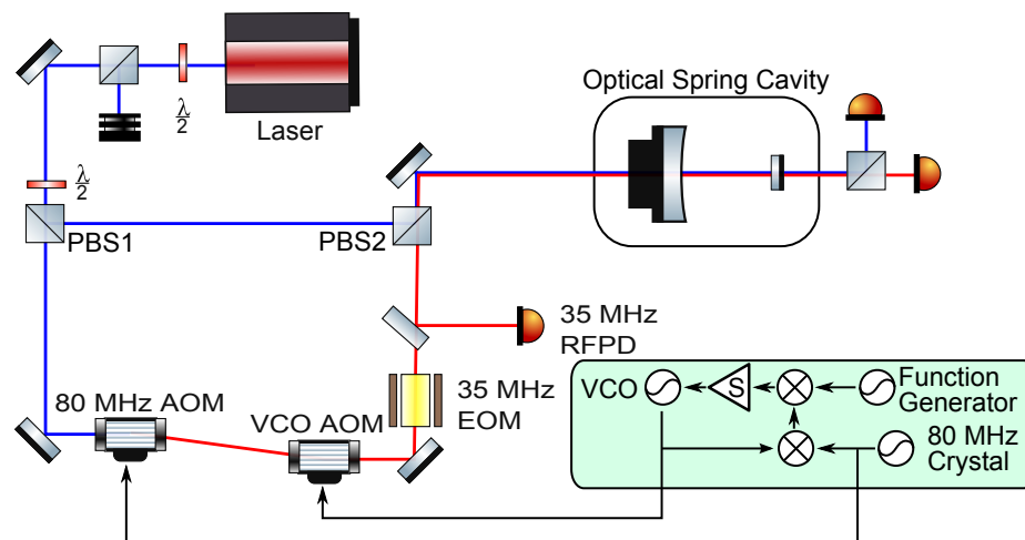
Figure 18 : There are two main control loops in an optical spring system. The first is the subcarrier servo, (green box, lower right) which detunes the subcarrier a set frequency from the carrier. The second controls the laser frequency and the trap cavity input coupler to lock the cavity.
