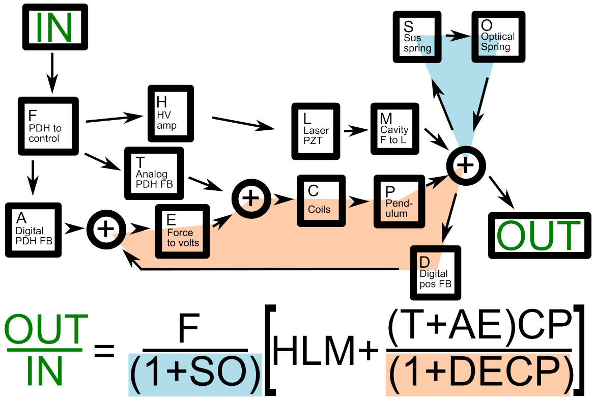
Figure 24 : Block diagram of the open loop transfer function for trap locking and operation. Two closed loops (OS and DECP) are highlighted in blue and red, respectively.
