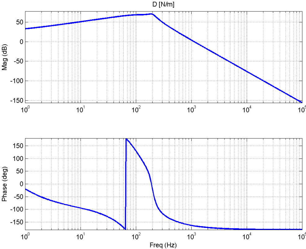
Figure 25 : D1, the transfer function from the position of optic 1, the input coupler, to a digital drive force.
