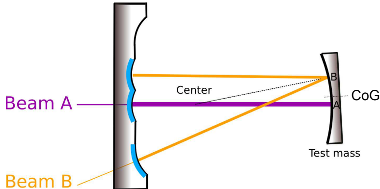
Figure 6 : In this sketch the main purple (beam A ) optical axis hits the test mirror at point A , slightly displaced from the center of gravity (CoG), such that it still corresponds mainly to the length degree of freedom. Thus the second orange (beam B ) optical axis, which hits the test mirror closer to the edge at point B , needs much less power to balance the total DC torque. In our test setup the large input coupler is a composite mirror. It is 600 times more massive than the small mirror. The choice of a V-shaped beam B results in a more practical spot separation on the input coupler.
