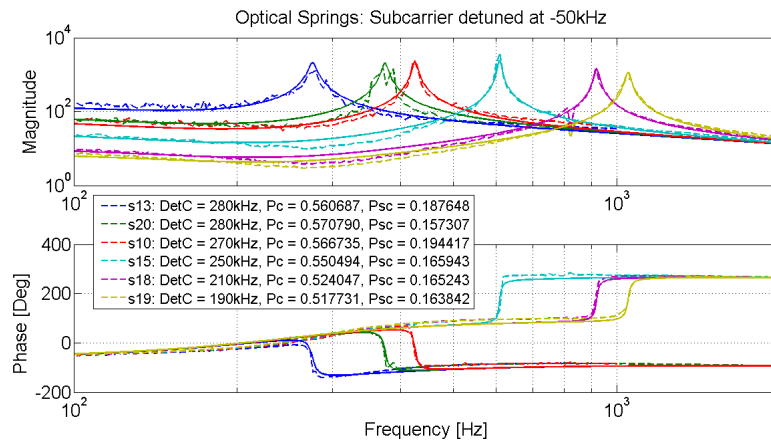
Figure 31 : Open loop TF of the system with several different carrier detunings. Changing the carrier detuning changes the resonant frequency of the springs and their stability. Included are both measurements and corresponding models.
