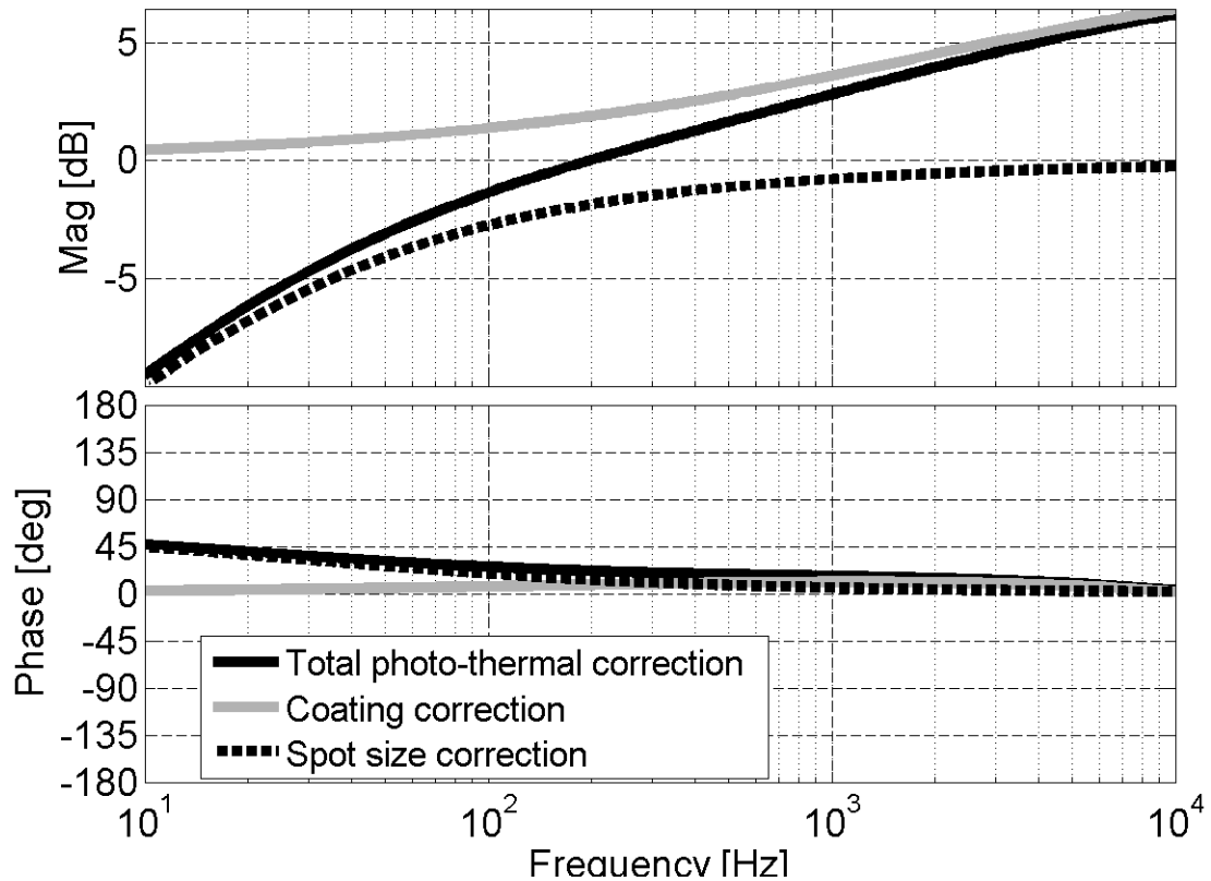
Figure 32 : Correction factors for the photo-thermal transfer function of a fused silica mirror with a dielectric coating (solid black). The solid grey trace is the coating correction for a 13-doublet \lambda/4 coating. The dashed black trace shows the effect of a Gaussian beam spot with w = 161 \mu\text{m} radius. To get the full transfer function, multiply with equation 5.5, adding an overall 1/f shape. The calculation is based on material parameters show in table 5.
