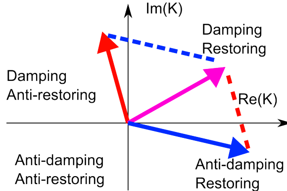
Figure 4 : We can add two unstable optical springs to make a system that is statically and dynamically stable. Note: this picture only makes sense in the low-frequency regime.
