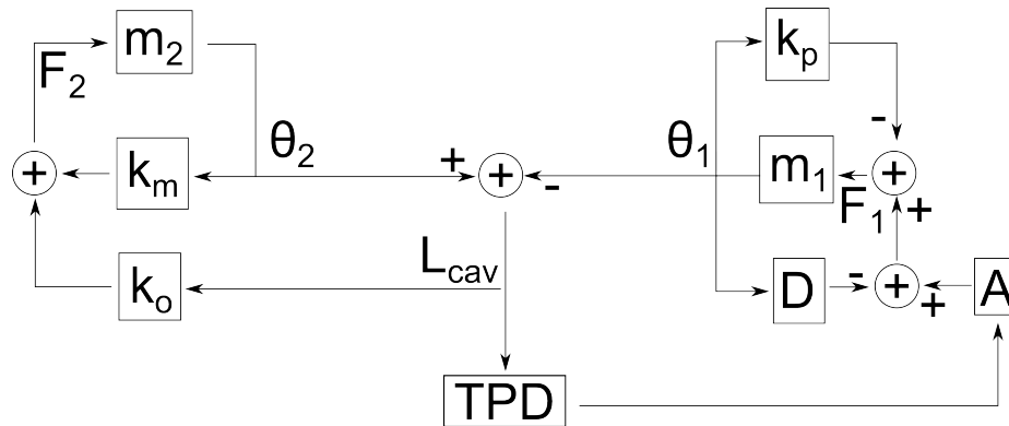
Figure 40 : Control loop structure for side cavity. Transmitted power is fed into yaw control for the input coupler.
