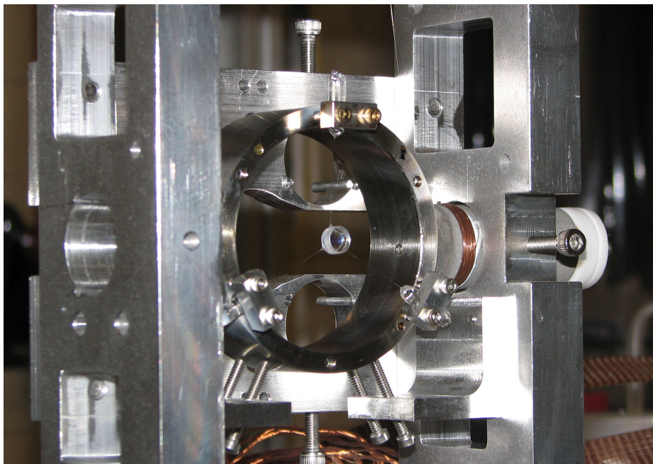
Figure 33 : A picture of the small end mirror suspended from a steel ring by glass fibers. The ring is suspended from a small optics suspension (SOS) with tungsten wire. The SOS provides DC alignment control while allowing the mirror to move freely above the 18Hz resonance of the fiber suspension. The end of the fiber is a small glass nub attached to the mirror with epoxy. This produces a fairly high suspension Q of about 5 \cdot 10^5 . The resulting contribution of damping in the opto-mechanical spring is insignificant compared to the damping from the optical field.
