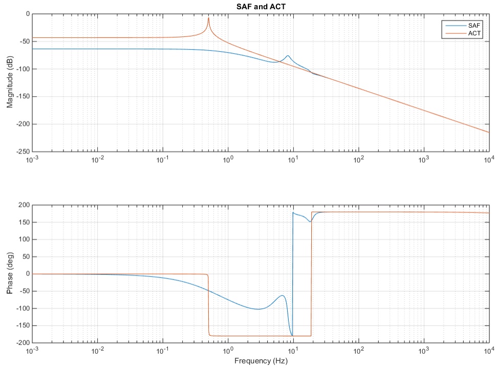
Figure 48 : The actuation function ( ACF ) and spring actuation function ( SAF = CLG \times ACF ) of the proposed angular control scheme. The actuation function includes the yaw pendulum behavior ( 1/f^2 ) of the mass and the yaw resonant frequency (chosen to be 0.5 Hz) of the ETM.
