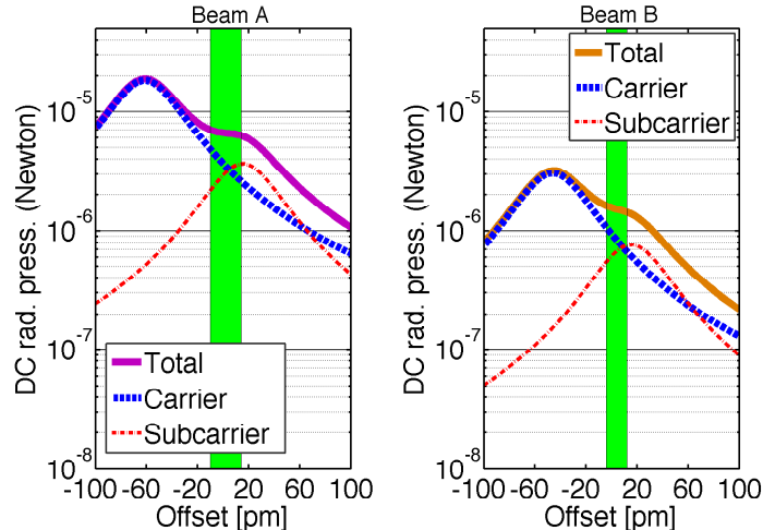
Figure 9 : Static carrier and subcarrier build-up (calibrated in radiation pressure force) as a function of the respective cavity position. Also shown in purple and orange are the total radiation pressure forces of the two cavities. Using the stability testing method from Sec. 2.4.2 we find that the trap is both statically and dynamically stable in the green shaded area. With the chosen model parameters those regions are about 20 picometers wide.
