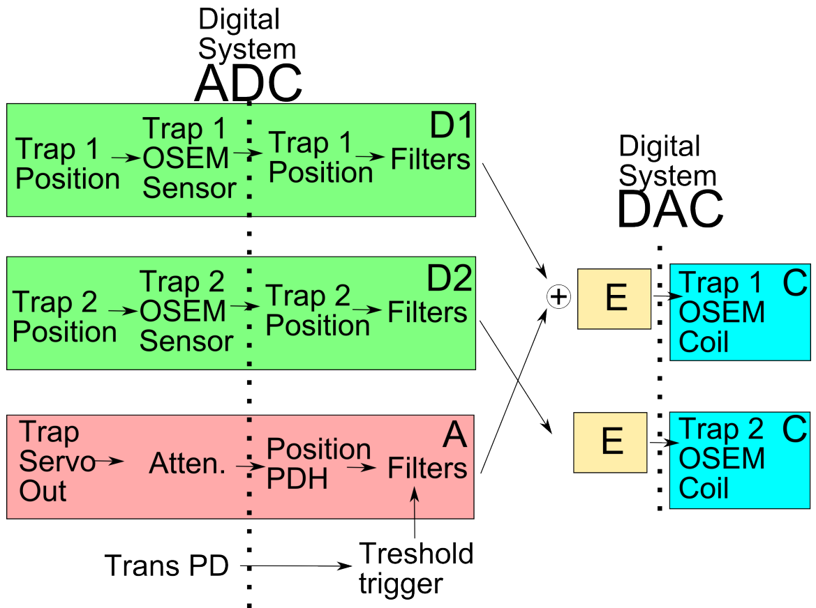
Figure 23 : Digital parts of the locking loop. These parts are responsible for the slow feedback to the OSEM coils. The yaw and optical lever inputs are not relevant to the longitudinal trap.
