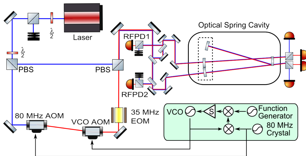
Figure 39 : Layout of the angular trap cavity experiment. The light from the laser is split into the carrier and subcarrier paths with a polarizing beam splitter (PBS), with a ratio determined by the \lambda/2 plate. The subcarrier path is frequency shifted by two AOMs under the control of the subcarrier servo then recombined with the carrier with another PBS. The co-aligned mode-matched beams are then split into main and side paths, which enter the trap cavity. The main beam has a straight optical path and is read out in transmission by broadband photodiodes and in reflection by RFPD1. The side beam has a folded optical path and is read out in transmission by broadband photodiodes and in reflection by RFPD2. We can use the 35 MHz modulation from the EOM with the two RFPDs in a PDH scheme to read out the cavity lengths or lock the cavities.
