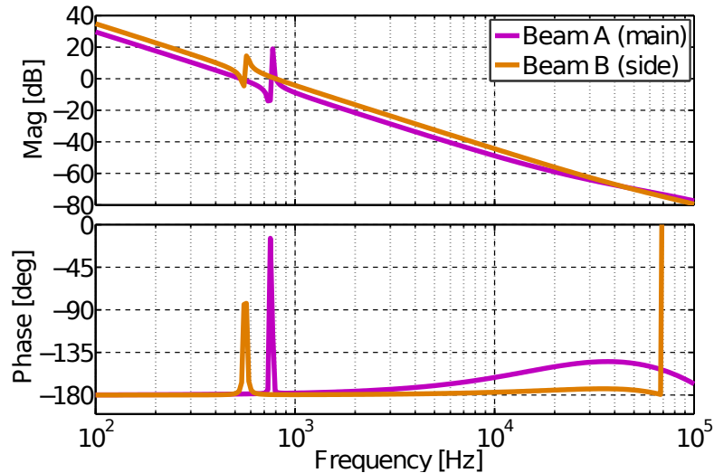
Figure 8 : Open loop gain (OLG) for the main and side cavity. The respective other loop is closed, and shows up as a resonance in the OLG. Note that, despite multiple unity gain crossings, both loops are stable because the resonances effectively implement a lead filter and the OLG avoids the critical point -1. Thus the dynamic interplay between multiple trapping beams on one payload does not introduce an instability.
