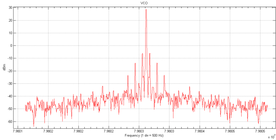
Figure 21 : Spectrum of the locked VCO. The sidebands are likely caused by the function generator.
