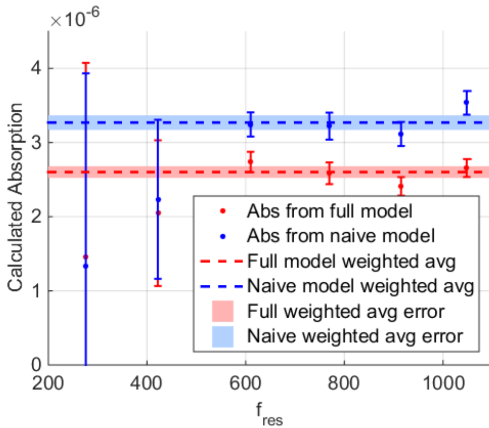
Figure 36 : Absorption fit for naive and full models. The full model absorption is consistent with a constant absorption of 2.60 \pm 0.08 ppm. The naive 1/f model predicts 3.27 \pm 0.10 ppm. The transfer function data for the lowest two resonant frequencies was significantly noisier. Also, at lower frequencies the photo-thermal effect has a smaller effect on the total optical spring. Both effects result in the larger error bars at low frequencies.
