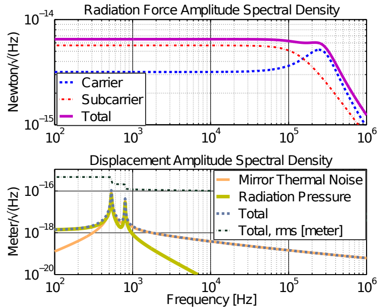
Figure 10 : (Top) Radiation force amplitude spectral density for the dual-carrier optical spring used in beam A of the above example. The subcarrier dominates the noise at low frequency, but the higher-power carrier contributes more at high frequencies. Also note that if we choose the same free spectral range for the two carriers, there would be an additional beat note at the difference frequency of 310 kHz. (Bottom) Radiation pressure and thermal noise displacement amplitude spectral density. The radiation pressure noise is calculated using the optomechanical response given in Eq. (2.27). The thermal noise is based on a theoretical calculation described in [29], [33]. Since seismic and suspension thermal noise depend on the experimental implementation, they are not shown, but they would also be suppressed by the optical spring closed loop response. The residual rms motion due to the shown noise sources is less than 10^{-3} picometers. With the total rms motion smaller than the 20 picometer stability band shown in Fig. 9, the two cavities will remain locked purely due to the radiation pressure trapping force.
