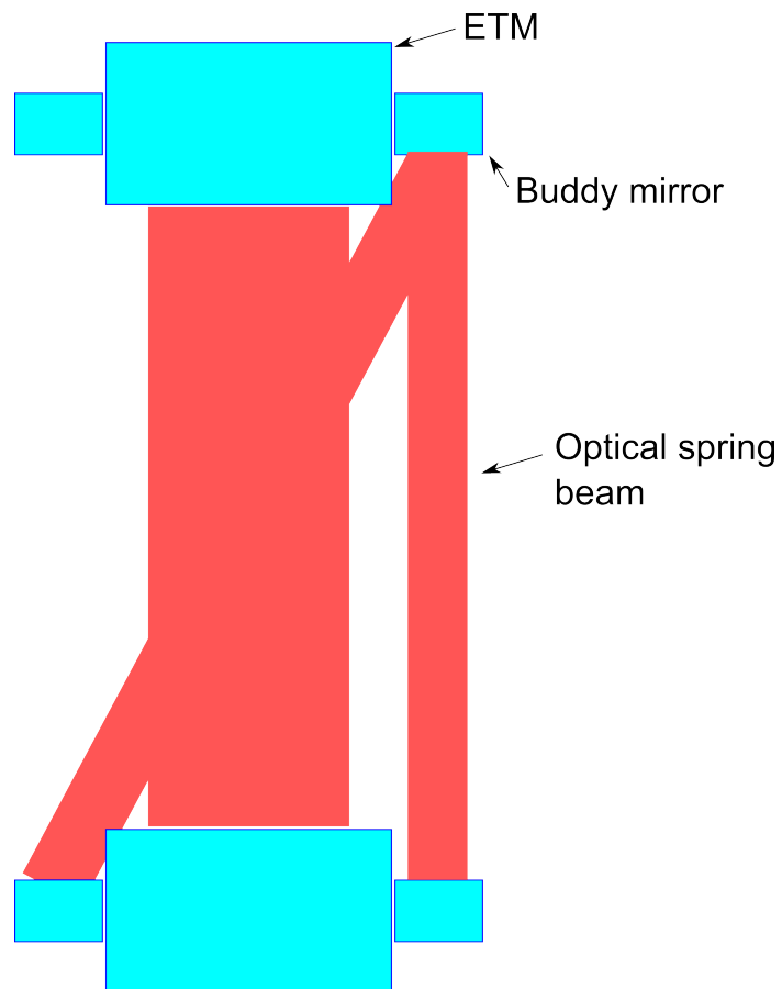
Figure 46 : Diagram of a folded cavity 4km angular control scheme. This configuration relies on 'Buddy' mirrors attached to the side of the test masses.
