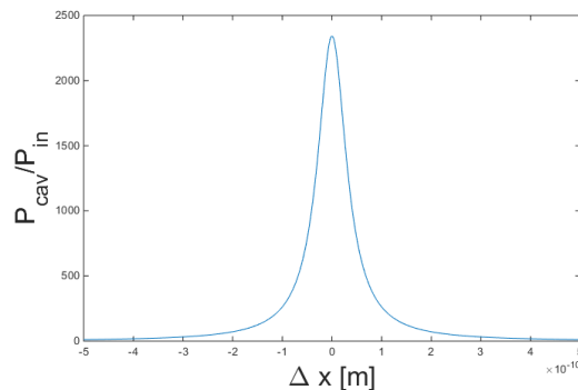
Figure 2 : Optical power in a critically coupled cavity near resonance. The height of the peak is determined by the reflectivities of the two mirrors and the input power. When the cavity is close to but not on resonance, power scales approximately linearly with the cavity length.
