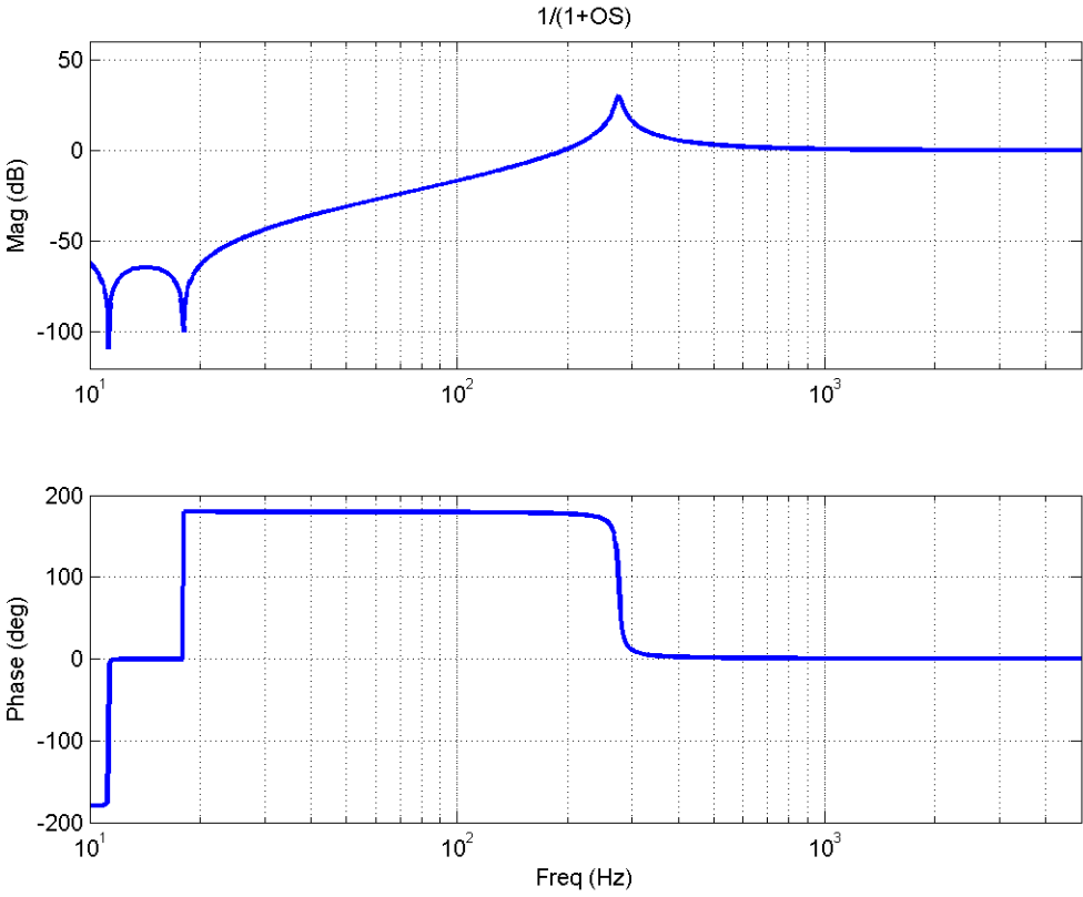
Figure 28 : Plot of the closed loop behavior of the optical spring and the glass suspension.
