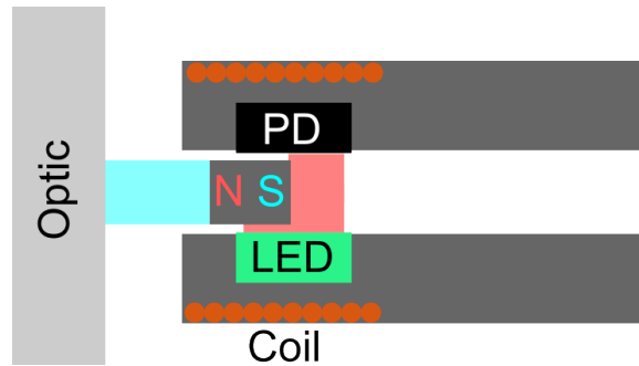
Figure 16 : Layout of an Optical Sensing Electro-Magnet (OSEM). Optic motion is sensed when the magnet changes the amount of light from the light emitting diode (LED) that gets to the photodiode (PD). The coils can be driven to move the magnet and thus the optic.
