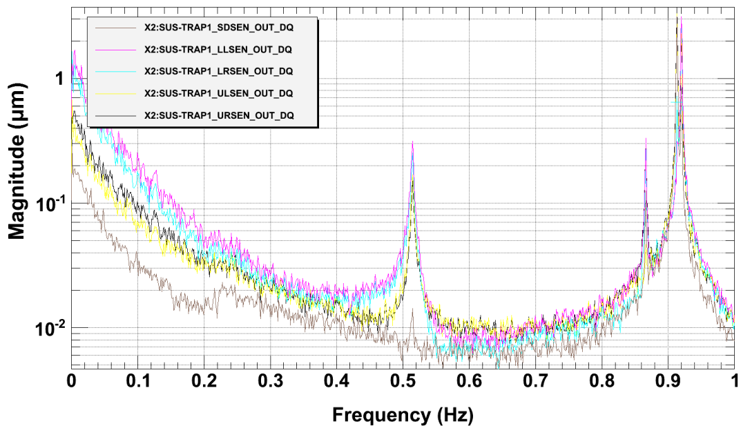
Figure 17 : Spectrum showing the modes of the input coupler. Modes from low to high are: Pitch (0.511 Hz), Yaw (0.866 Hz), Side (0.911 Hz), and Position (0.918 Hz).
