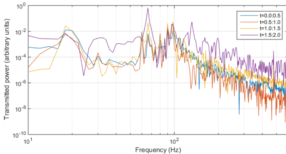
Figure 42 : Spectrum of the two second lock shown in fig 41. The four traces for show spectra taken every 0.5 seconds from t = 0 to t = 2.0 . The line at 66 Hz rings up over time. In the last trace, we can see the harmonics of 66 Hz also rung up.
