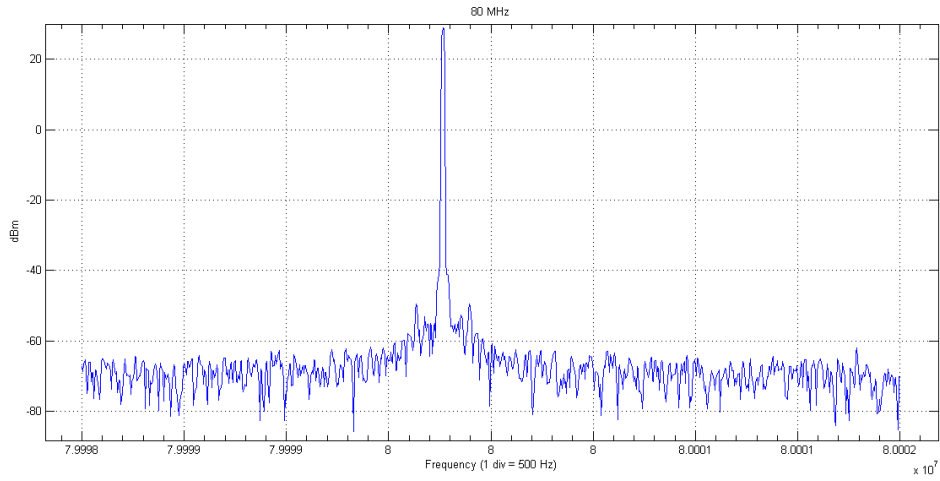
Figure 20 : Spectrum of the 80 MHz crystal oscillator around 80 MHz.
