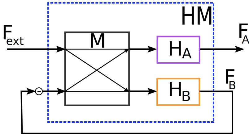
Figure 7 : Block diagram of beam A and beam B . The transfer function F_A/F_{ext} is equal to OL_A from Eq. (2.13). Each loop affects the other resulting in cross terms present in the matrix HM . M and H_{A,B} are the transfer functions of the mechanical system and the optical springs of beam A and B , respectively.
