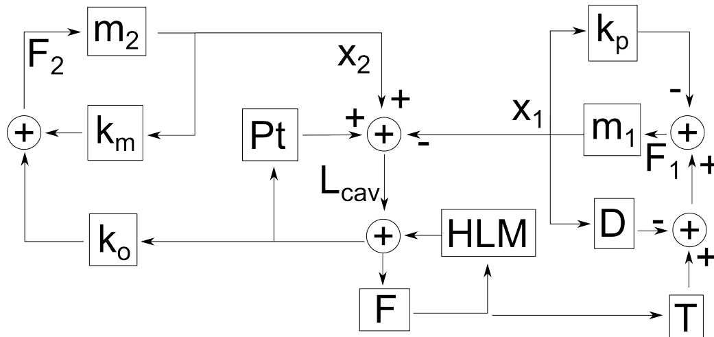
Figure 30 : Loop diagram for a single degree of freedom, including photothermal feedback, Pt . The optical spring loop on the left side ( k_o , k_m , and m_2 ) is affected by the photothermal effect ( Pt ). We measure the behavior of the optical spring by measuring the open loop transfer function of the system at F , then dividing out the transfer functions of the control system ( HLM , T , D , etc.). This leaves us with the closed loop transfer function of the optical spring with the photothermal effect.
