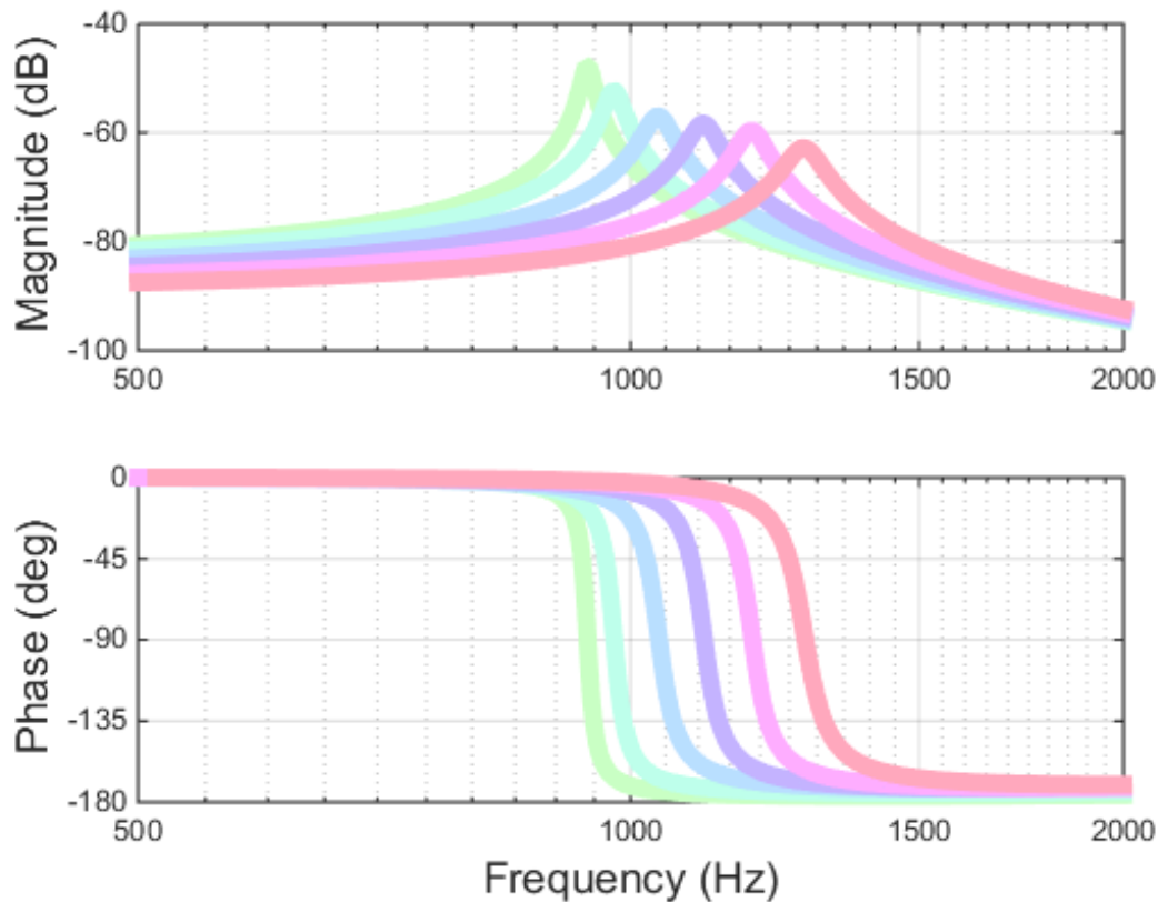
Figure 38 : Stable single-carrier optical springs (no sub-carrier) with modified coating - the first coating layer is 20.5 wavelength thick. See text for details. The six traces otherwise have the same parameters as the best-fit optical springs in figure 35.
