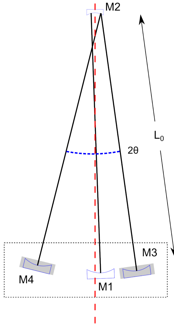
Figure 44 : Layout of the angular trap cavity. Light enters through mirrors M1 and M3. The angle \theta of the folded cavity is measured from the normal of M1.
