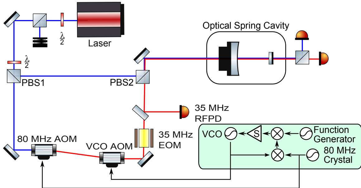
Figure 34 : A schematic layout of the optical trap experiment. The light from the laser is split into the carrier and subcarrier paths at PBS1, with a ratio determined by the \lambda/2 plate. The subcarrier path is frequency shifted by two AOMs under the control of the subcarrier servo (described in detail in Section 5.5.3), then recombined with the carrier at PBS2. The co-aligned mode-matched beams enter the cavity, then are individually monitored at the output. We can use the 35 MHz EOM and RFPD in a PDH scheme to read out the cavity length or lock the cavity.
