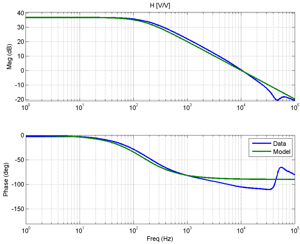
Figure 29 : HV amplifier transfer function. Includes a high-frequency bypass to increase feedback bandwidth.
