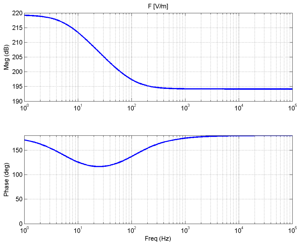
Figure 26 : Calculated trap servo TF. The main components are a 1 kHz lowpass filter and a user-adjustable gain.
