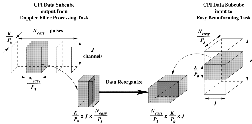
Fig. 8. Data redistribution from Doppler filter processing task to easy beamforming task. CPI data subcube of size (K/P_0) \times J \times N_{easy}/P_3 is reorganized to subcube of size (N_{easy}/P_3) \times (K/P_0) \times J before sending from one processor in Doppler filtering processing task to another in easy beamforming task.
