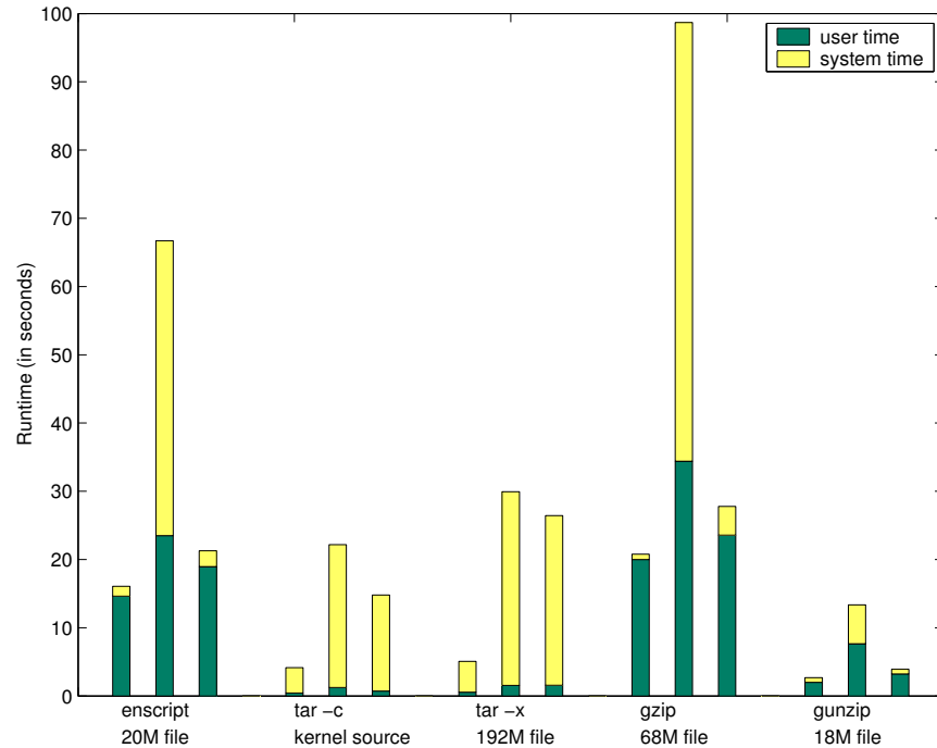
Fig. 3. overhead of the waypoint-based access monitor. For every group, the left side bar shows the time of running the original program; the middle bar shows its running time under waypoint-based access monitoring for all functions; and the right side bar shows the result with monitoring only functions that invoke dangerous system calls.
