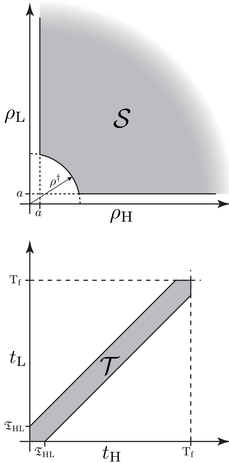
Figure 11 : The regions of integration in \rho , and time for a network of two detectors, H and L.
