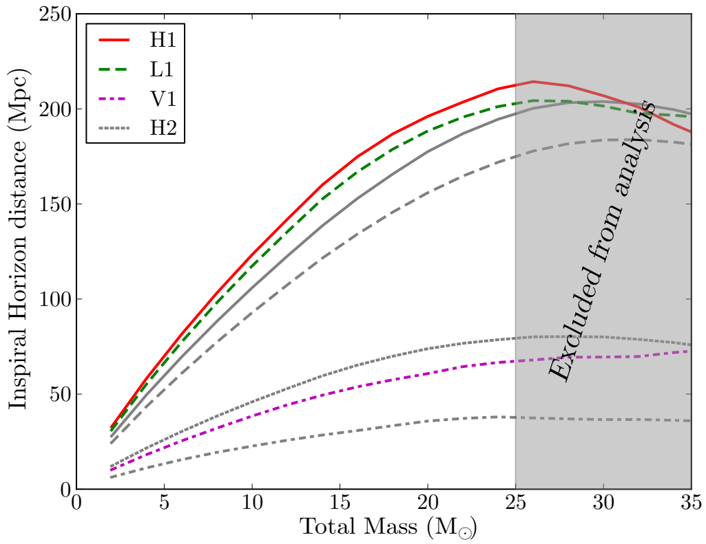
Figure 45 : Average inspiral range of S6D. Shaded region indicates the mass range that was excluded in the low mass search for this period. Ranges were computed using the same method as in Figure 7.2.
