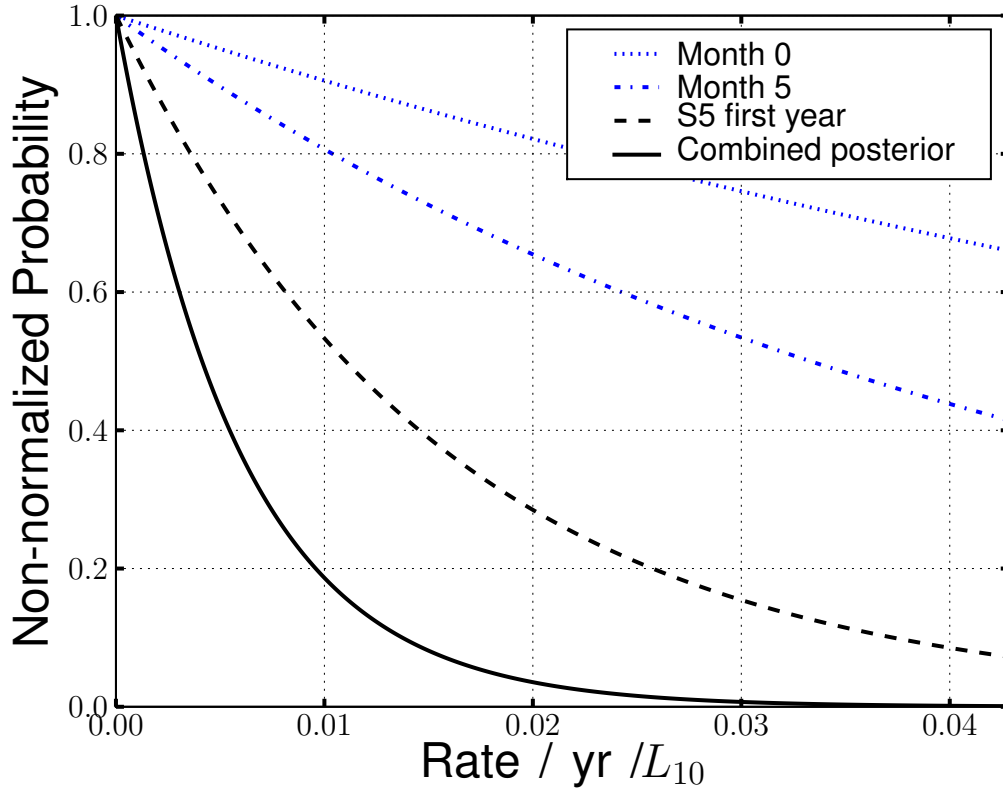
Figure 39 : The posterior distribution for the rate of BNS coalescences. The dashed black curve shows the rate computed in [9]. The solid black curve shows the result of this search using the previous analysis as a prior. The figure also shows the rate distributions for two of the individual months computed using a uniform prior. The improvement from month 0 to month 5 is due to increasing detector sensitivity during this search.
