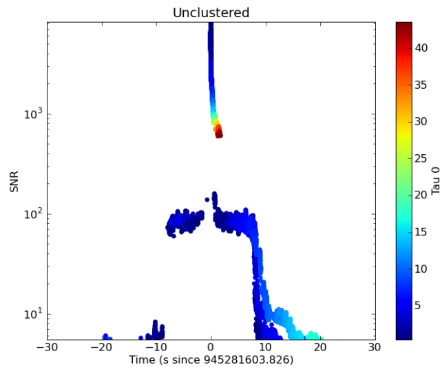
Figure 59 : The unclustered triggers created by the spike glitch shown in 7.3.2 when passed through lalapps_inspiral .
