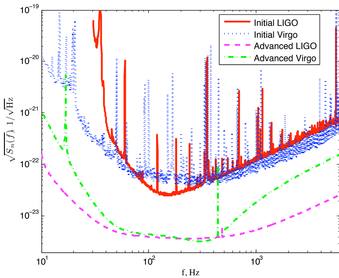
Figure 7 : Amplitude spectral densities of initial LIGO and Virgo detectors. Shown also are the expected noise curves for advanced LIGO and Virgo. Figure originally published in [1].
