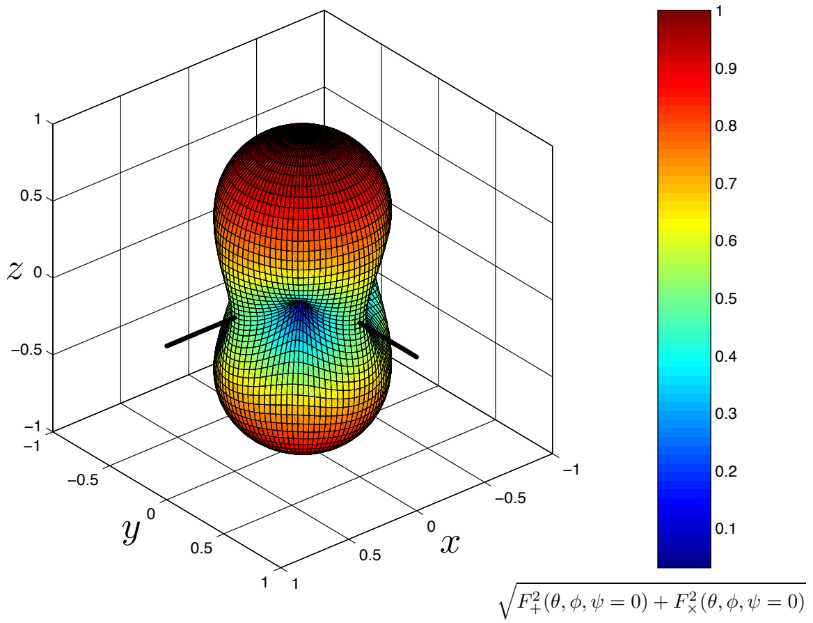
Figure 5 : The antenna pattern of an interferometer (IFO). The arms of the IFO are plotted for reference. Figure originally published in [2].
