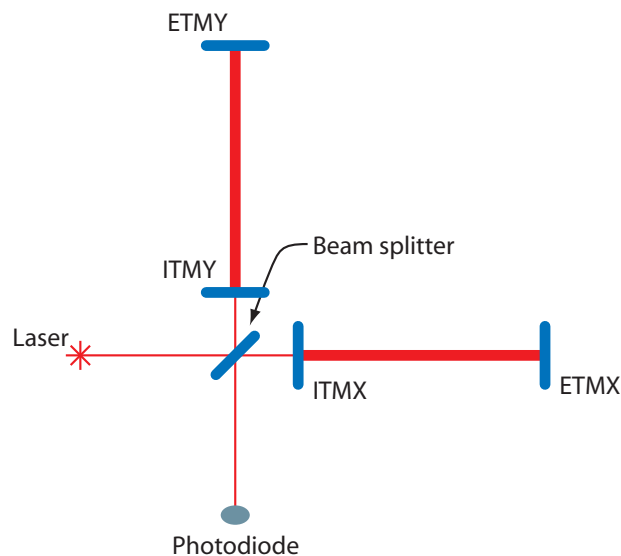
Figure 6 : Schematic of an interferometer with a Fabry-Perot cavity. Originally published in [2].
