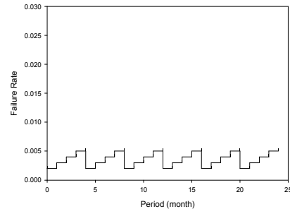
Fig. 8-3 Case 1 Unit 3 Failure Rate Profile
