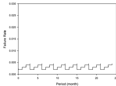
Fig. 8-2 Case 1 Unit 2 Failure Rate Profile
