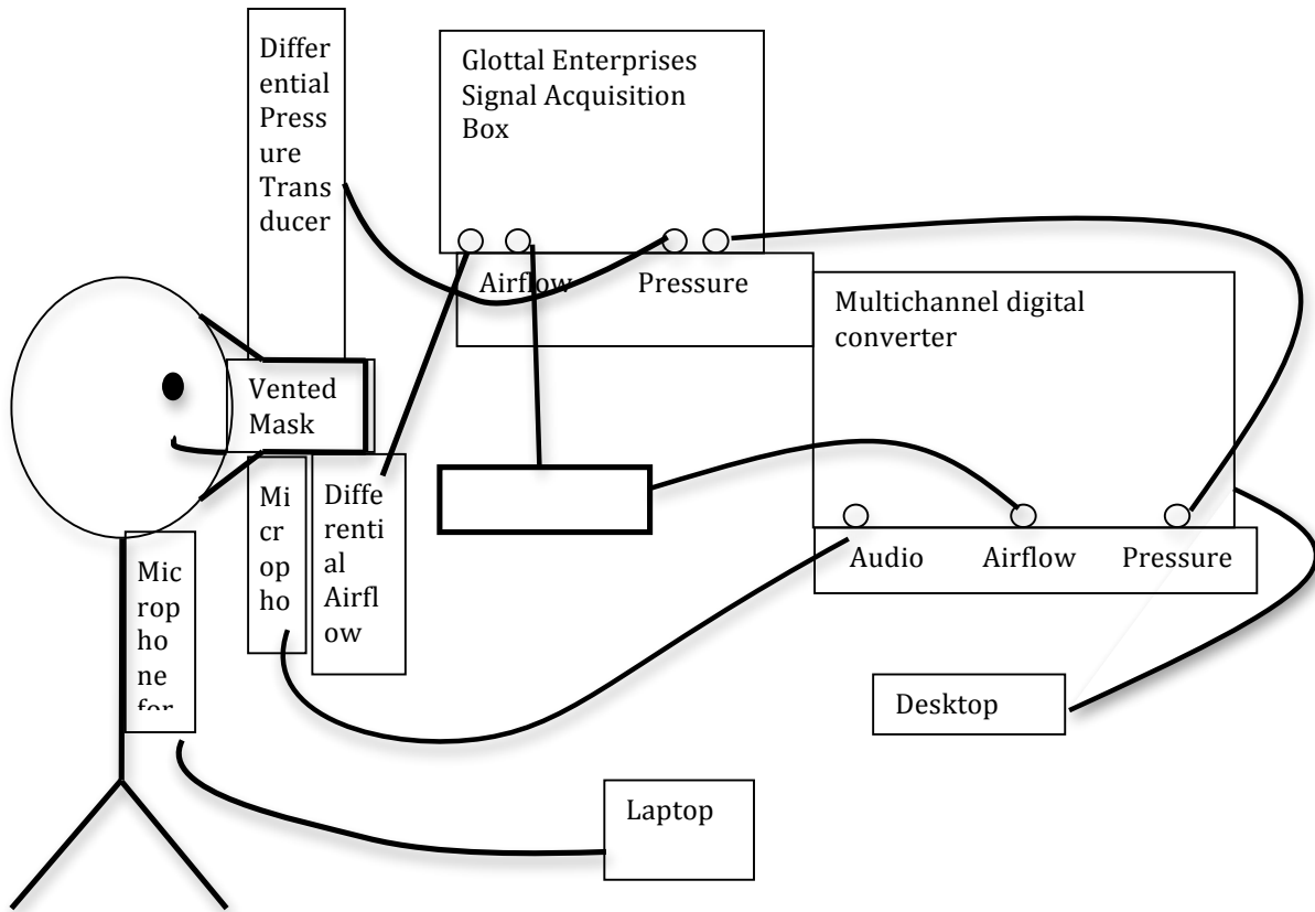
Figure 1: Instrumentation
