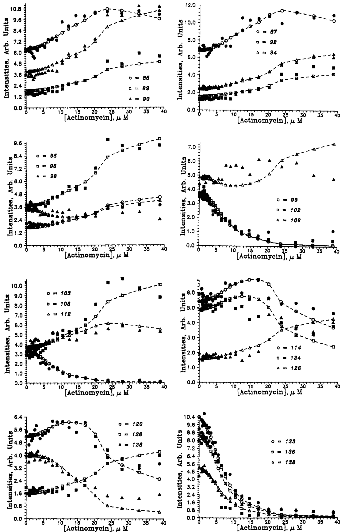
FIGURE 6: Footprinting plots from the A-label gel for selected sites in the region 85–138 of the fragment. Solid symbols are experimental gel spot intensities; fits calculated according to our best model (column III of Table III) are shown as open symbols and dashed lines. Sites 89, 90, 95, 96, and 108 are enhancement sites. Sites 133, 136, and 138 show strong drug binding.
