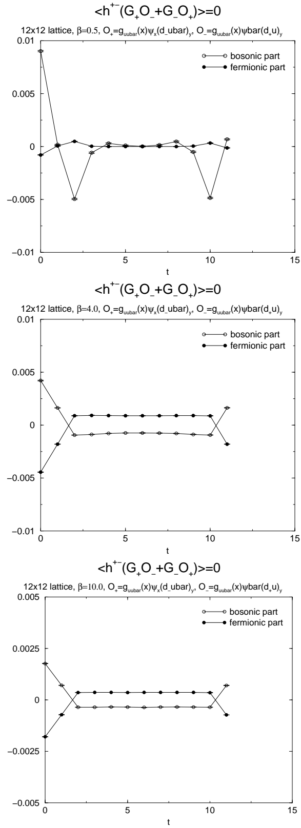
Figure 7: \langle h^{+-}(G_+O_- + G_-O_+) \rangle = 0 for 12 \times 12 lattice
