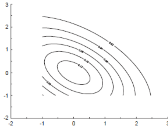
Fig. 1. Standard bivariate truncated normal contour, \sigma_{12} = -0.5 , c = -1 .
