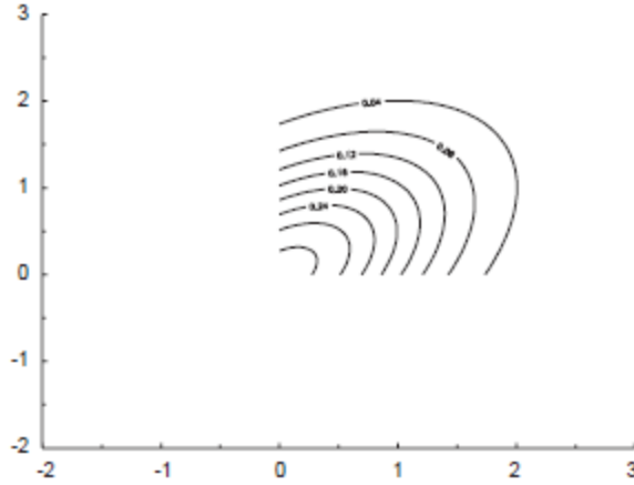
Fig. 4. Standard bivariate truncated normal contour, \sigma_{12} = 0.5 , \mathbf{c} = \mathbf{0} .
