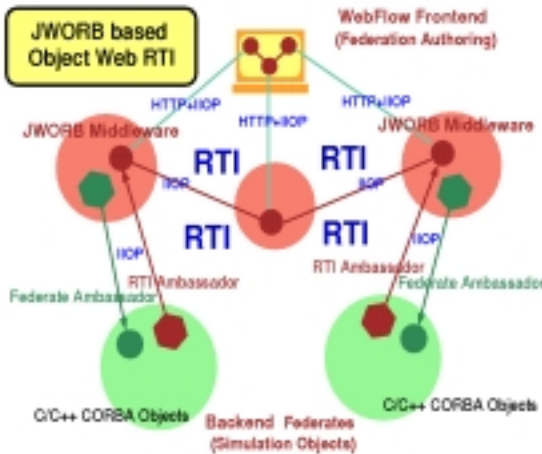
Figure 13: Overall architecture of the Object Web RTI - a JWORB based RTI prototype recently developed at NPAC
