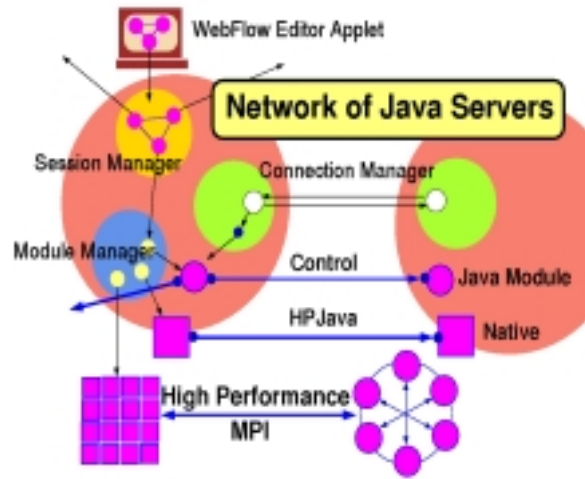
Figure 19: Overall Architecture of the 3-tier WebFlow model with the visual editor applet in tier-1, a mesh of Java Web Servers in tier 2 (including WebFlow Session Manager, Module Manager and Connection Manager servlets), and (high performance) computational modules in tier-3.
