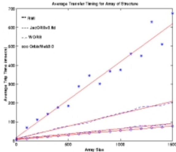
Figure 10: IIOP communication performance for transferring a variable size array of structures by four Java ORBs: JacORB, JWORB, OrbixWeb and RMI. Poor RMI performance is due to the object serialization overhead, absent in the IIOP/CDR protocol.
