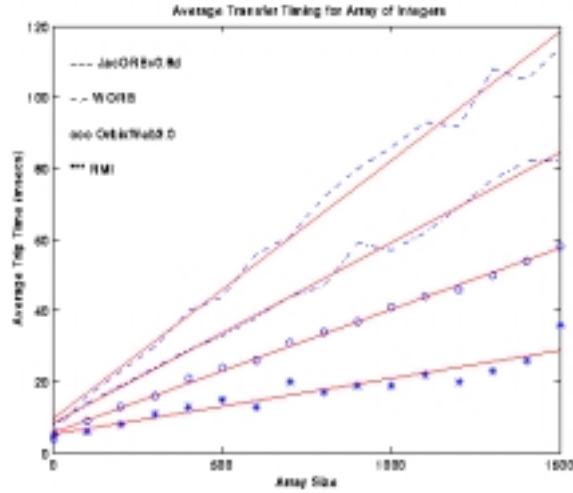
Figure 9: IIOP communication performance for variable size integer array transfer by four Java ORBs: JacORB, JWORB, OrbixWeb and RMI. As seen, initial JWORB performance is reasonable and further optimizations are under way. RMI appears to be faster here than all IIOP based models.
