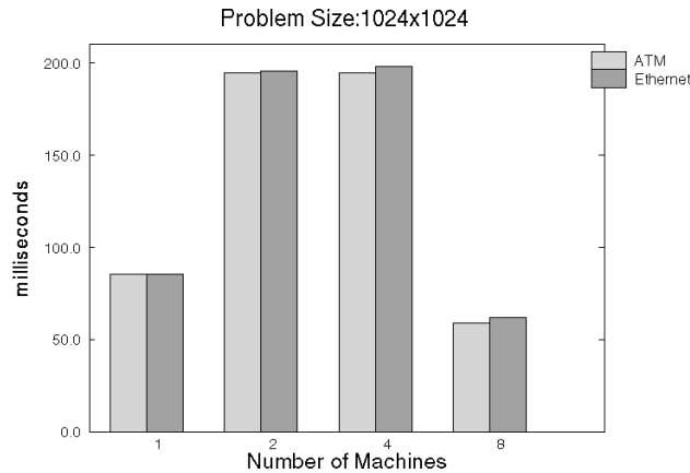
Figure 9: Execution Time of Matrix Multiplication Task Using p4
