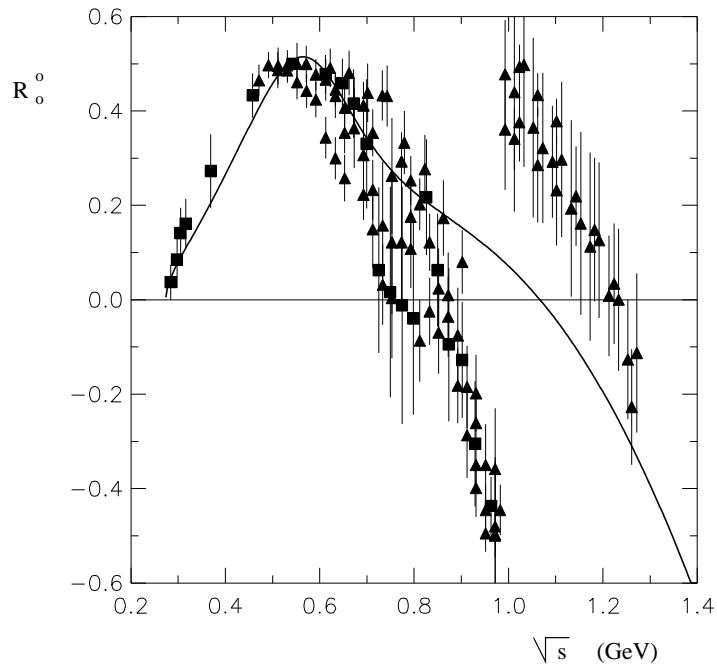
Figure 2: The solid line is the current algebra + \rho + \sigma result for R_0^0 . The experimental points, in this and succeeding figures, are extracted from the phase shifts using eq. (A.6) and actually correspond to R_0^0/\eta_0^0 . ( \square ) are extracted from the data of Ref. [8] while ( \triangle ) are extracted from the data of Ref. [9]. The predicted R_0^0 is small around the 1 GeV region.
