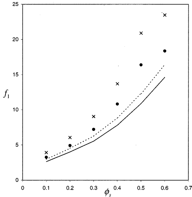
FIG. 3. The coefficient f_1 as a function of \phi_s for the random arrays of spheres. The filled circles and solid line correspond, respectively, to the exact results and the approximate relation for the case of \delta = \delta_0 at low gas flow rates. The crosses and the dashed lines are the corresponding results for the distribution \delta = \delta_0(\sin \theta)^{-2/3} .
