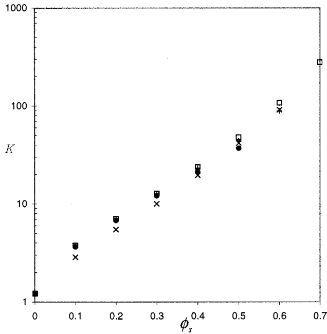
FIG. 1. The dry bed drag coefficient K as a function of \phi_s . The filled circles are the results for the simple cubic arrays, pluses for the body-centered cubic arrays, squares for the face-centered cubic arrays, and crosses for the random arrays of spheres.
