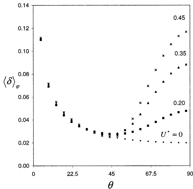
FIG. 11. The azimuthal angle-averaged film thickness, \langle \delta \rangle_\varphi , as a function of \theta at various U^* .
