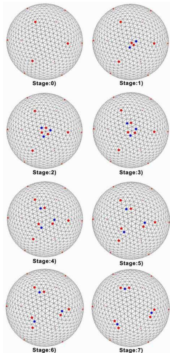
FIG. 9: (Color online) We first consider an initial lattice with icosahedron symmetry, an (8, 3) icosadeltahedral lattice (stage 0). The I_2 interstitial is generated by adding one extra particle (stage 1), which evolves into a I_3 interstitial (stage 2). The curvature-driven unbinding of dislocations starts—the decay of an interstitial (stages 3 and 4). Individual dislocation glides towards the nearest isolated disclination (stage 5 and 6). Each dislocation binds to a disclination to form three miniscars (stage 7). The results are obtained from the java applet developed in Ref. [23], according to the procedure described in the Appendix.
