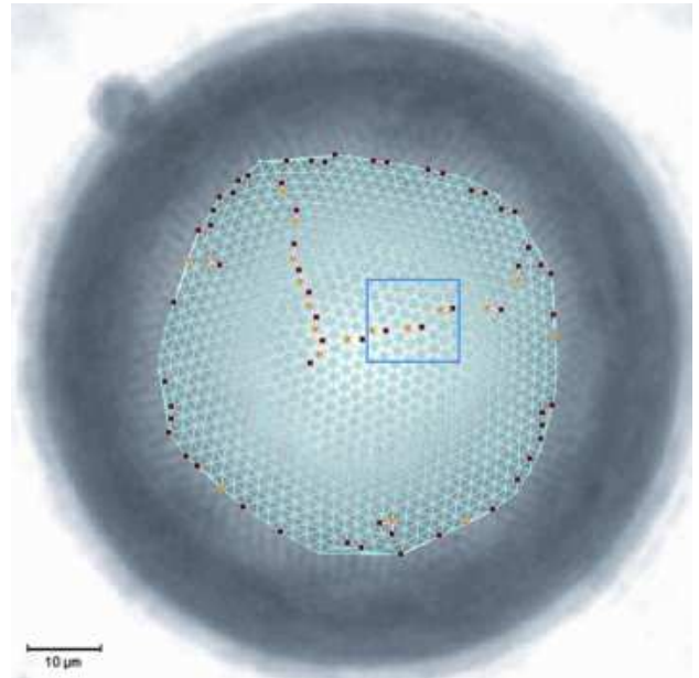
FIG. 1: (Color online) A light microscope image, reproduced from [12], of a water droplet with an 85 \mu\text{m} diameter and 1.9 \mu\text{m} mean particle spacing ( R/a \approx 22 ). Fivefold (+1) disclinations are colored red, Sevenfold (-1) disclinations are colored yellow, and tightly bound five to seven pairs represent dislocations. The three dislocations whose dynamics are analyzed in this paper are displayed within the blue box.
