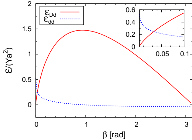
FIG. 5: (Color online) The Disclination-dislocation ( D-d ) and dislocation-dislocation ( d-d ) interaction energies as a function of defect separation \beta . The inset is a blowup of the short-distance region of the plot.
