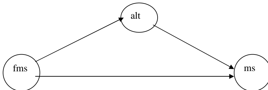
Fig. 4. Hypothesis 1 (path a: fms-alt; path b: alt-ms; path c: fms-ms)
