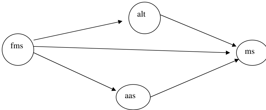
Fig. 7. Hypothesis 4: the overall model (path a: fms—alt; path b: alt—ms; path c: fms—ms; path d: fms—as; path e: as—ms; fms – fibromyalgia impact; ms – marital satisfaction; alt – alexithymia; as – adult attachment style)
