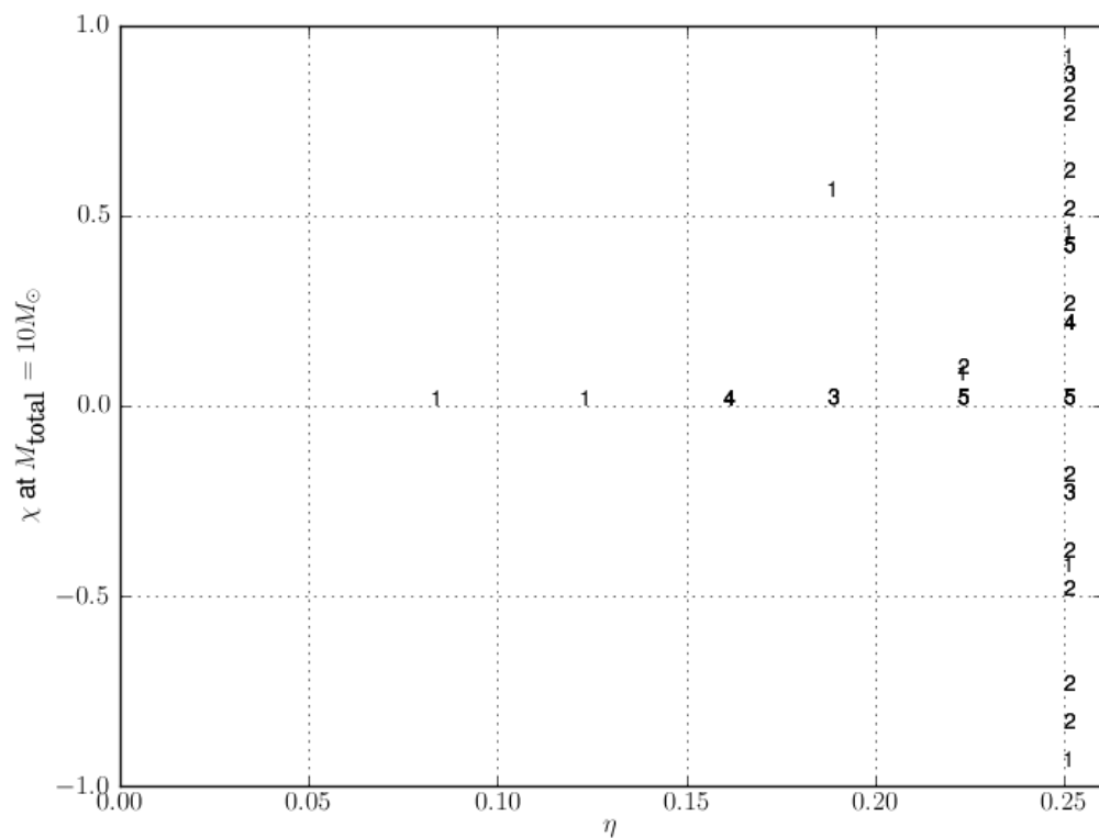
Figure 19 : Parameters of the NINJA-2 hybrid waveform submissions showing the symmetric mass ratio \eta = m_1 m_2 / (m_1 + m_2)^2 and dimensionless spin parameter \chi = (S_1/m_1 + S_2/m_2)/(m_1 + m_2) after scaling the waveforms to a reference total mass of 10 M_\odot . The numbers indicate how many distinct waveforms with the specified parameters were submitted.
