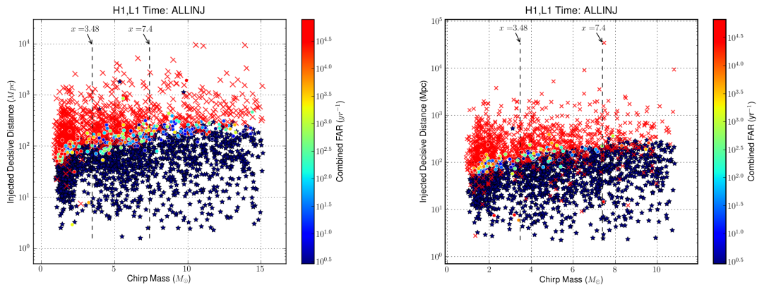
Figure 94 : Found and missed plots for simulated injection in two weeks of real noise. Results from the current code are on the left, the modified code (as described in the text) is on the right. The feature to focus on is found injections (blue dots) and missed injections (red crosses). There are many more missed injections using the modified code.
