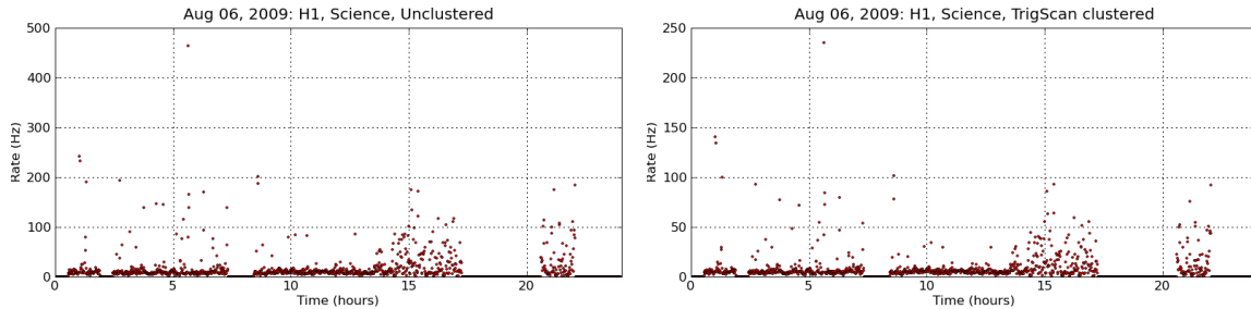
Figure 74 : Problematic times identified by daily ihope . The plot on the left shows the rate of triggers over the day without any clustering. Note the sudden jump in rate at 5:40. On the right, the same plot after clustering triggers with the trigscan algorithm. The overall rate has been reduced by about a factor of two, indicated by the different scales on the y axes. However, the rate remains high enough to cause problems.
