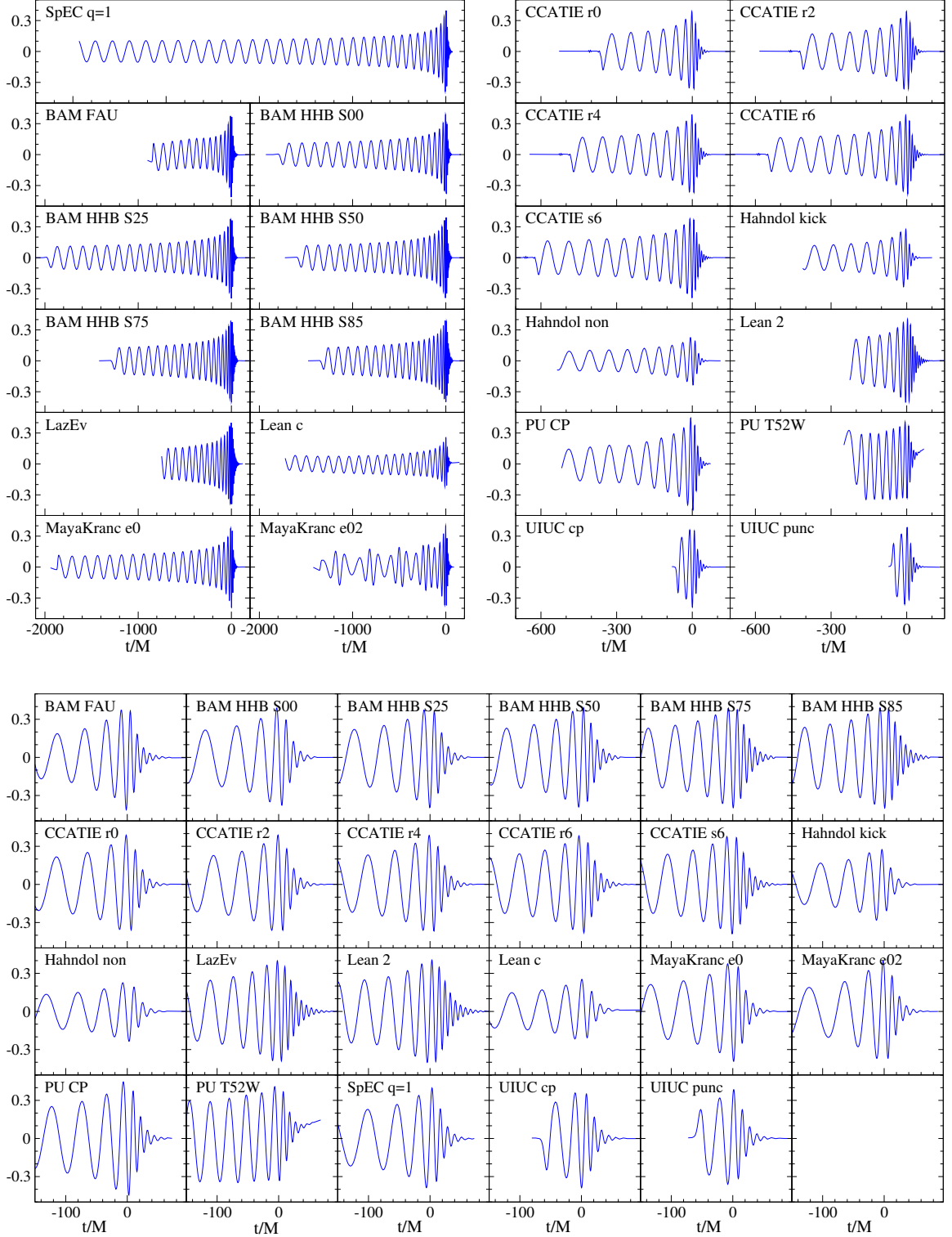
Figure 10 : Summary of all submitted numerical waveforms: r/M \text{Re}(h_{22}) . The x -axis shows time in units of M and the y -axis shows the real part of the (\ell, m) = (2, 2) component of the dimensionless wave strain rh = rh_+ - irh_\times . The top panels show the complete waveforms: the top-left panel includes waveforms that last more than about 700M , and the top-right panel includes waveforms shorter than about 700M . The bottom panel shows an enlargement of the merger phase for all waveforms.
