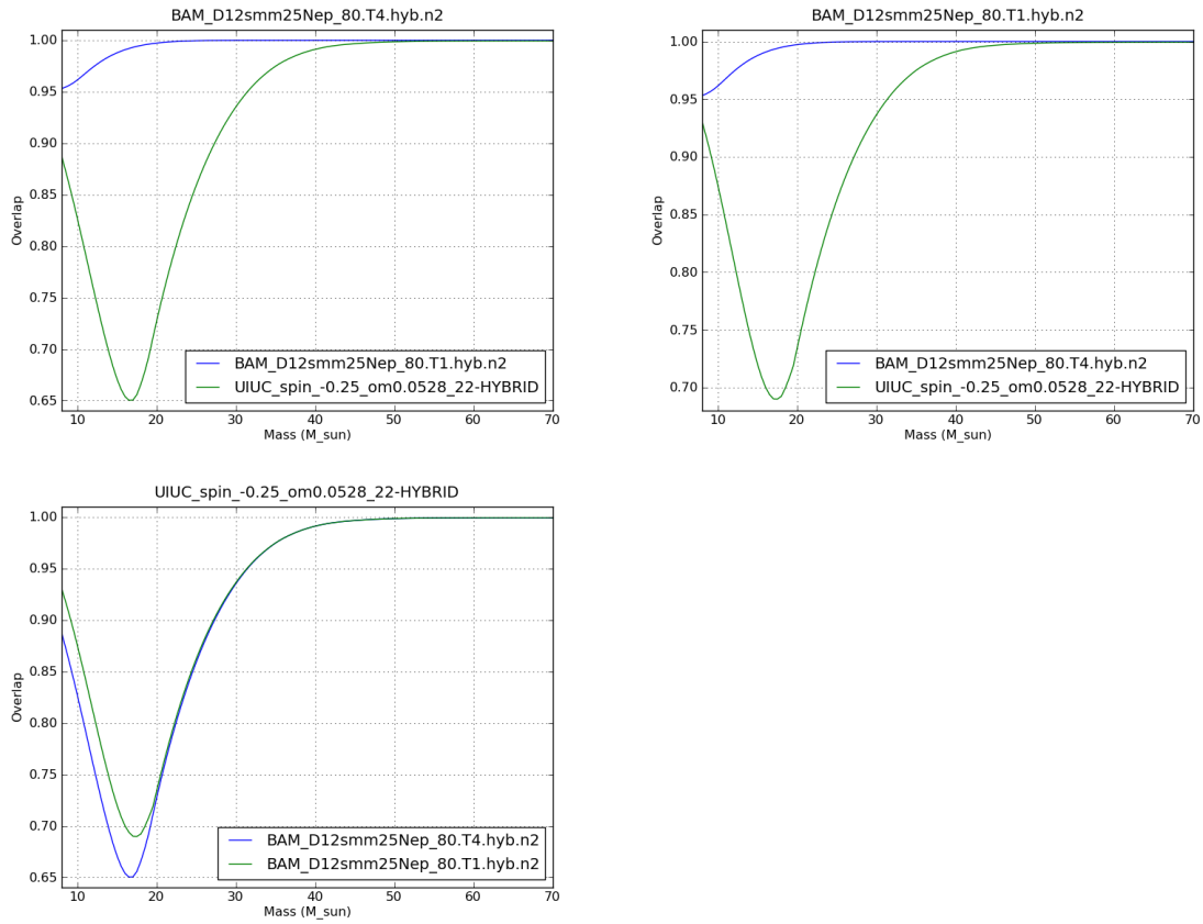
Figure 31 : Overlap plots for q = 1 S_{z1} = S_{z2} = -0.25
