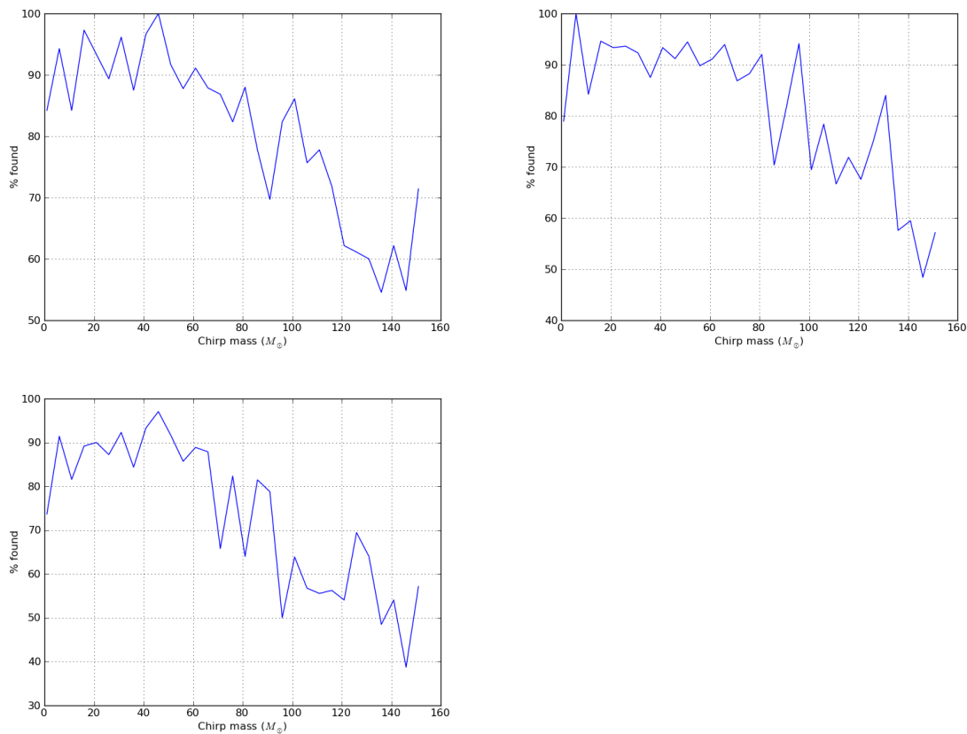
Figure 46 : Efficiencies of the high-mass pipeline as a function of mass. As can be seen in figure 45 the efficiencies decrease as mass increases. However, the scatter in these plots indicates that there are not enough injections to draw definitive conclusions.
