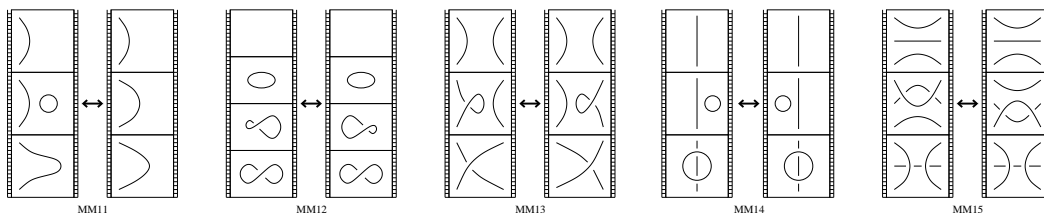
Figure 1.6: Type III moves.
