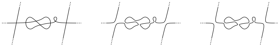
Figure 4.4: A knot projection, and two smoothings related by a state transposition.
