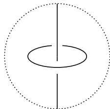
Figure 4.6: A (1,1) -tangle.
