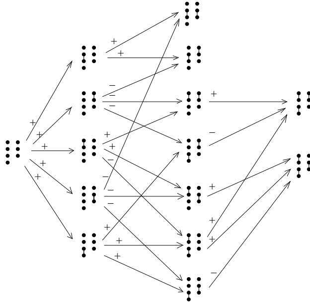
Figure 6.1: The graph \Gamma_{4,3} .
