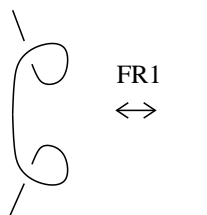
Figure 5.2: The framed Reidemeister move FR1.
