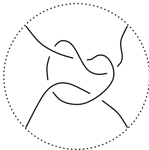
Figure 1.10: A tangle.
