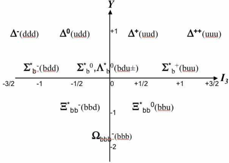
Figure 3: Spin \frac{3}{2} baryon decuplet representation of SU(3)_B .
