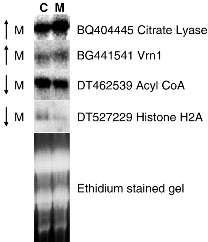
Figure 2. Northern analysis of four representative probes hybridized to total velvetleaf RNA isolated from plant grown in competition with corn (C) or in monoculture (M). Probes were from the designated genes (with both GenBank accession number and top BLAST hit); arrows indicate if the gene was predicted to be up-regulated or down-regulated in monoculture based on microarray data.
